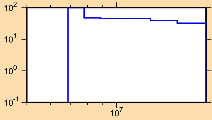
\Delta\sigma/\sigma vs. E for ^{211}\text{Ra}(n,2n)
