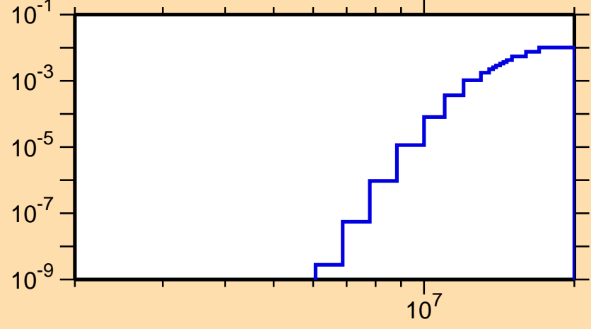
\sigma vs. E for ^{211}\text{Ra}(n,d)
