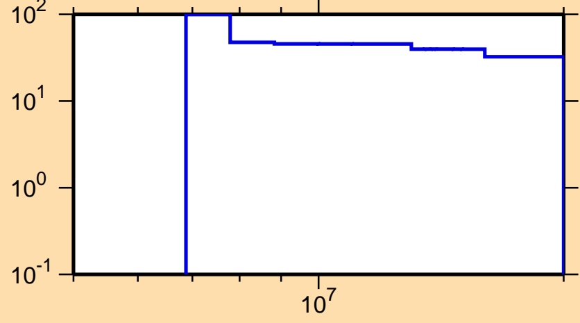
\Delta\sigma/\sigma vs. E for ^{211}\text{Ra}(n,2n)
