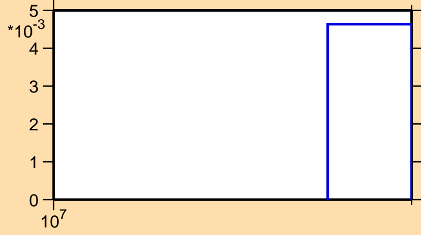
\sigma vs. E for ^{211}\text{Ra}(n,3n)
