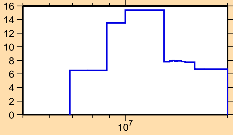
\Delta\sigma/\sigma vs. E for ^{211}\text{Ra}(n,\text{tot.})
