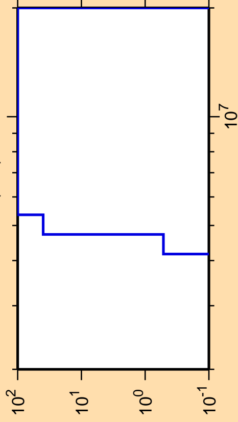
\Delta\sigma/\sigma vs. E for ^{211}\text{Ra}(n,d)
