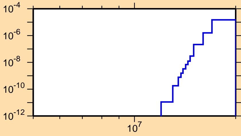
\sigma vs. E for ^{211}\text{Ra}(n,\text{nd})
