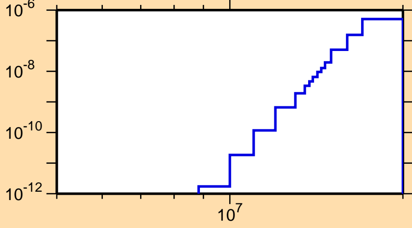
\sigma vs. E for ^{211}\text{Ra}(\text{mt } 45)
