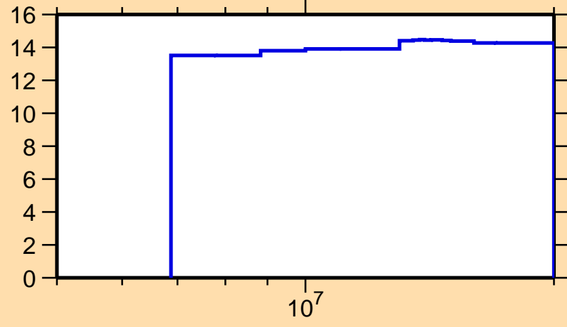
\Delta\sigma/\sigma vs. E for ^{211}\text{Ra}(n,\text{nonel.})
