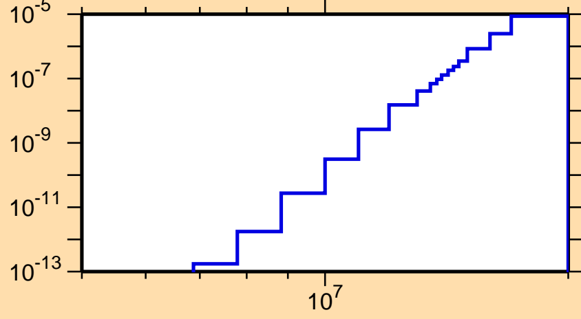
\sigma vs. E for ^{211}\text{Ra}(n,\text{He3})
