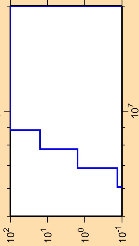
\Delta\sigma/\sigma vs. E for ^{211}\text{Ra}(n,\text{He3})
