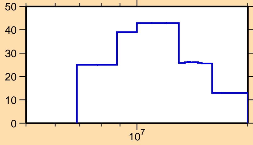
\Delta\sigma/\sigma vs. E for ^{211}\text{Ra}(n,\text{el.})
