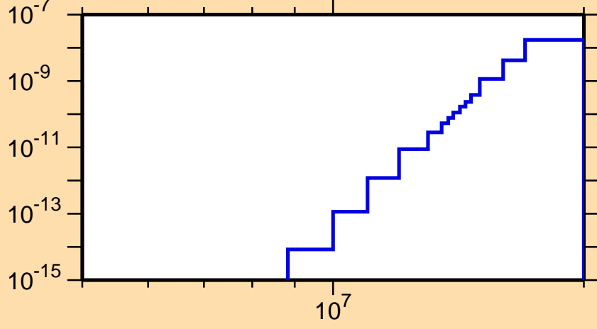
\sigma vs. E for ^{211}\text{Ra}(\text{mt117})
