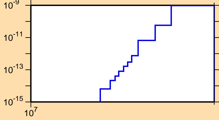
\sigma vs. E for ^{211}\text{Ra}(\text{mt } 34)
