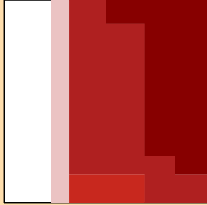
\Delta\sigma/\sigma vs. E for ^{211}\text{Ra}(n,2n)
