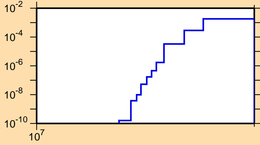
\sigma vs. E for ^{211}\text{Ra}(n,2np)
