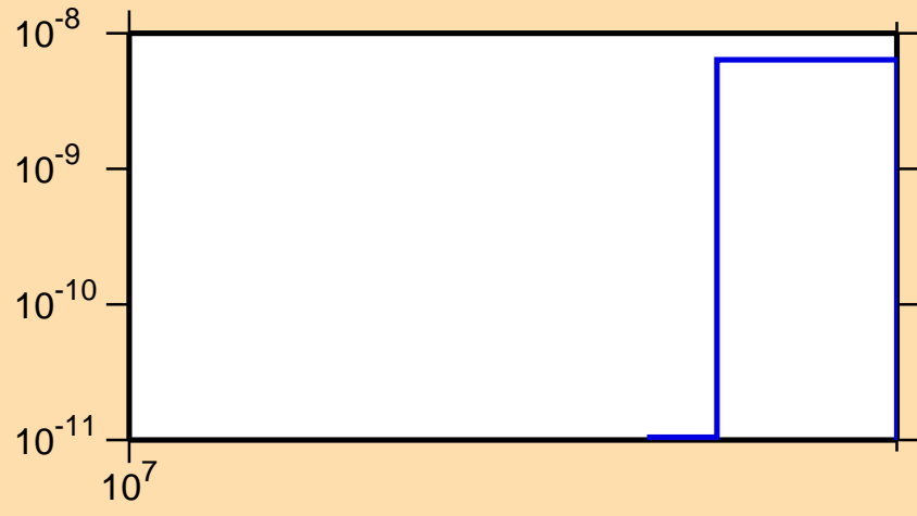
\sigma vs. E for ^{211}\text{Ra}(n,nt)
