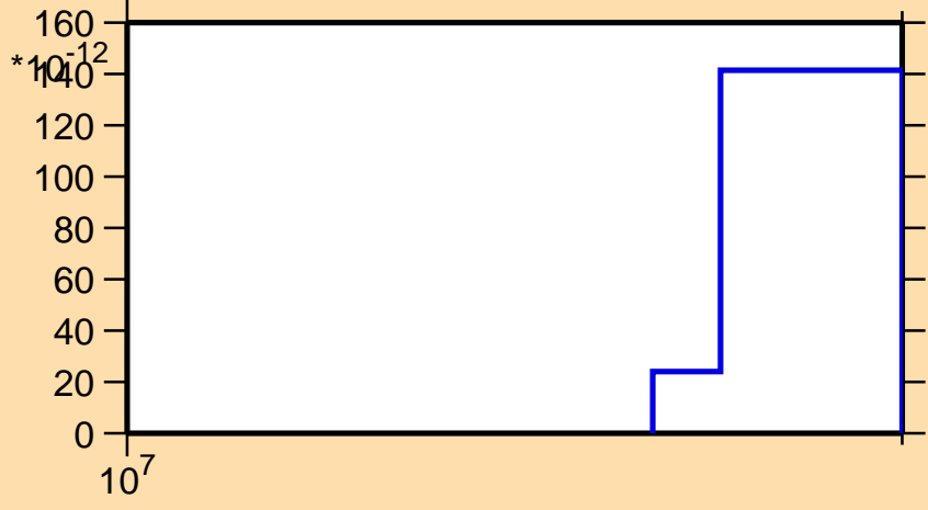
\sigma vs. E for ^{211}\text{Ra}(n,3n\alpha)
