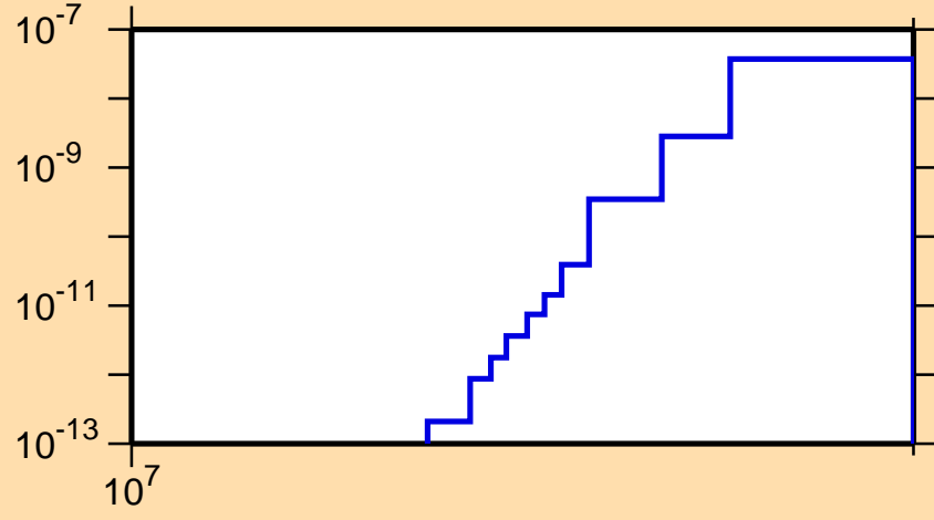
\sigma vs. E for ^{211}\text{Ra}(n,\text{pt})
