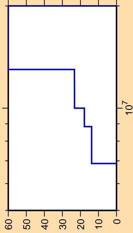
\Delta\sigma/\sigma vs. E for ^{211}\text{Ra}(n,n\text{cont.})
