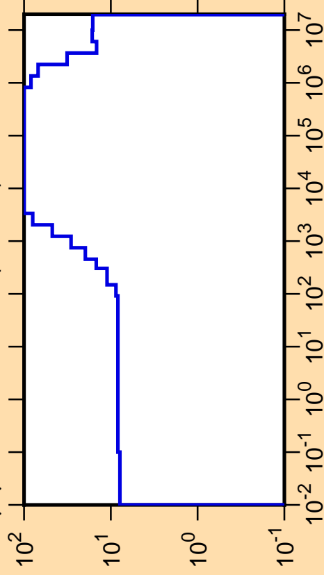
\Delta\mu/\mu vs. E for ^{211}\text{Ra}(\text{mt251})
