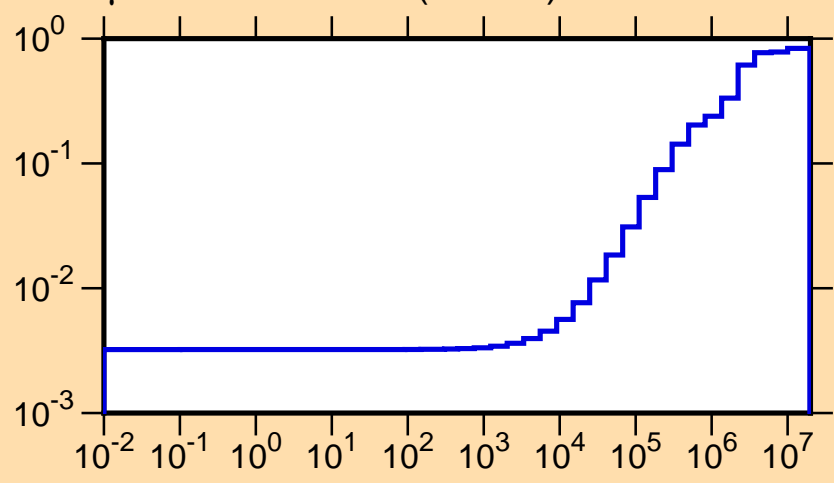
\mu vs. E for ^{211}\text{Ra}(\text{mt251})
