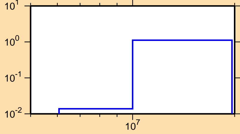
\sigma vs. E for ^{211}\text{Ra}(n,2n)
