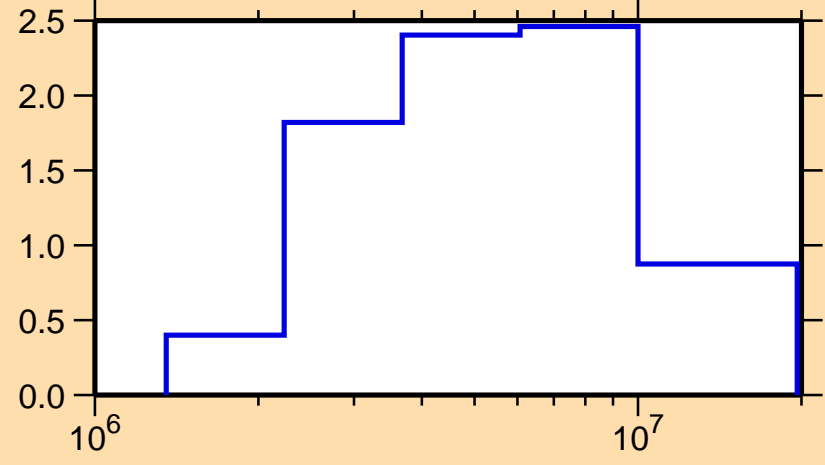
\sigma vs. E for ^{211}\text{Ra}(n,n\text{cont.})
