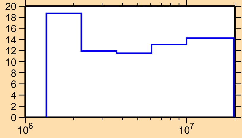
\Delta\sigma/\sigma vs. E for ^{211}\text{Ra}(n,n\text{onel.})
