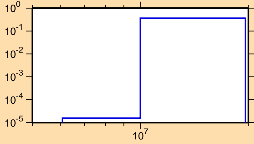
\sigma vs. E for ^{211}\text{Ra}(n,2n\alpha)
