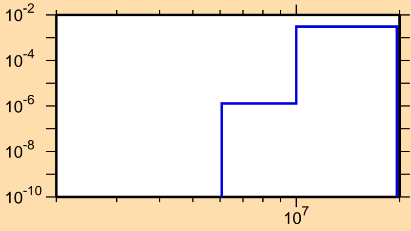
\sigma vs. E for ^{211}\text{Ra}(n,d)
