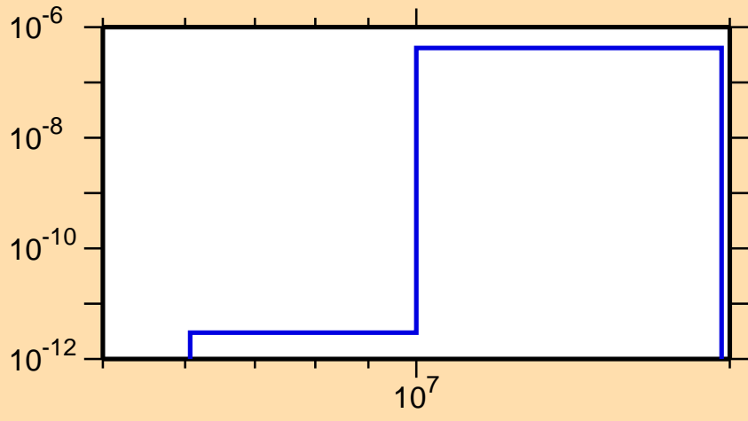
\sigma vs. E for ^{211}\text{Ra}(n,\text{He3})
