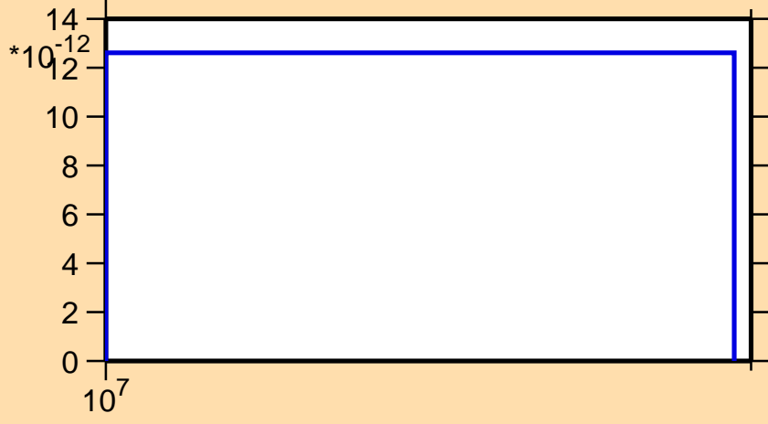
\sigma vs. E for ^{211}\text{Ra} (mt 34)
