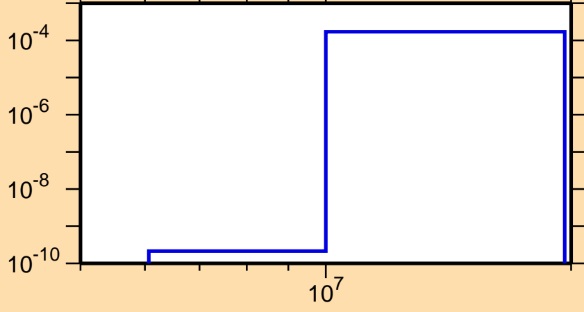
\sigma vs. E for ^{211}\text{Ra}(n,t)
