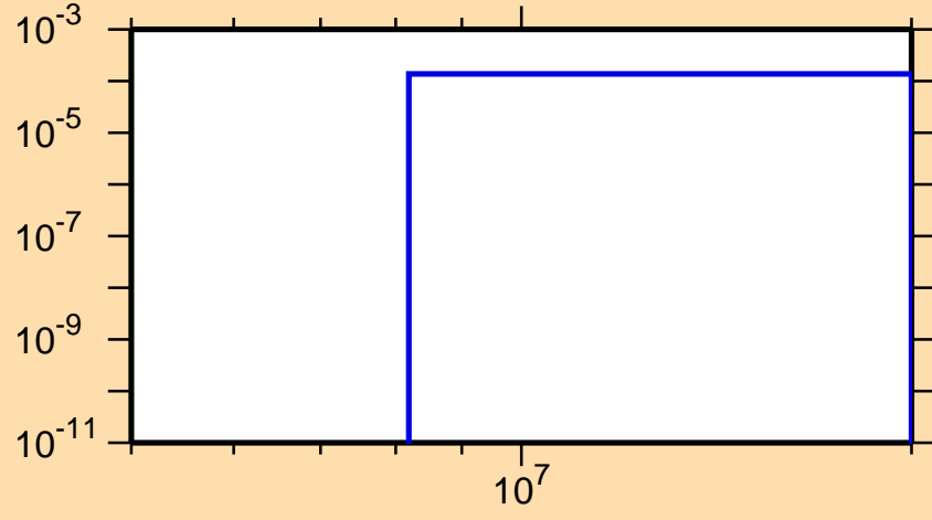
\sigma vs. E for ^{211}\text{Ra}(n,t)
