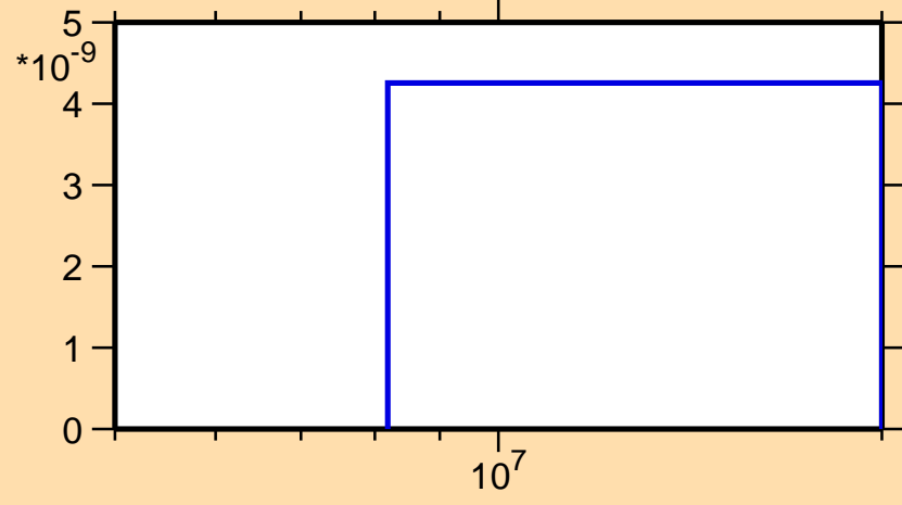
\sigma vs. E for ^{211}\text{Ra}(n,\text{pd})
