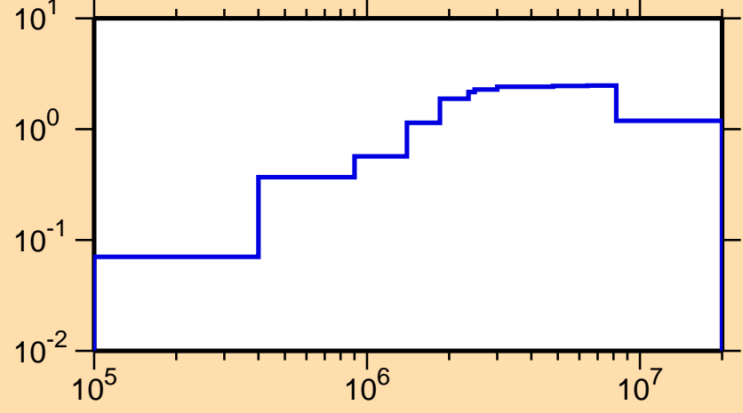
\sigma vs. E for ^{211}\text{Ra}(n,\text{inel.})
