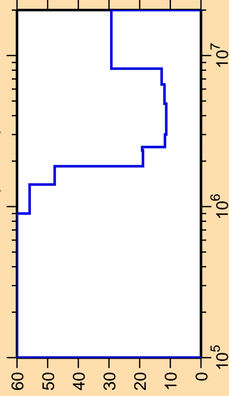
\Delta\sigma/\sigma vs. E for ^{211}\text{Ra}(n,\text{inel.})
