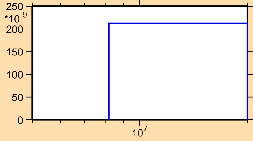
\sigma vs. E for ^{211}\text{Ra}(n,\text{nd})
