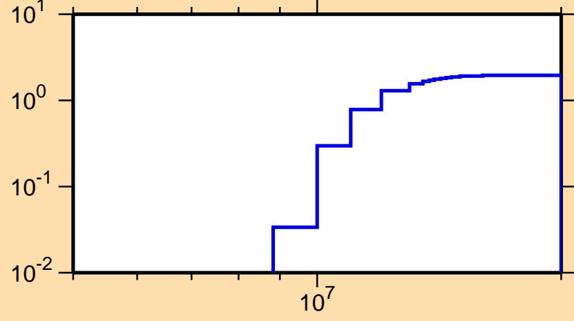
\sigma vs. E for ^{212}\text{Ra}(n,2n)
