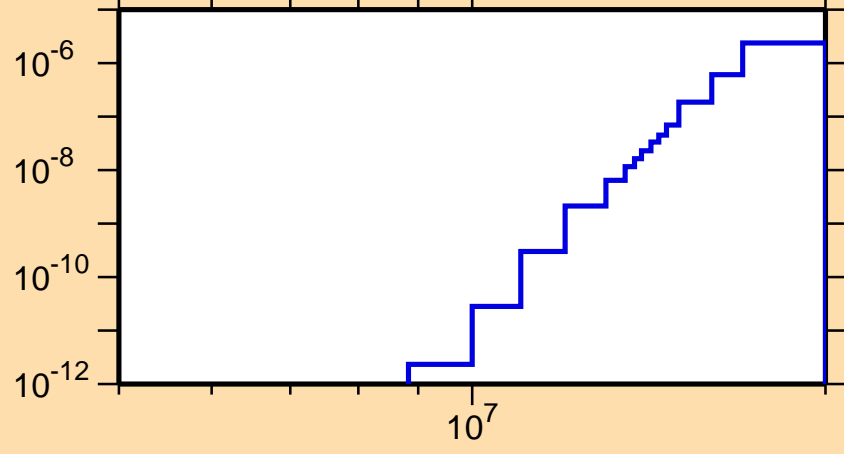
\sigma vs. E for ^{212}\text{Ra}(n,\text{He3})
