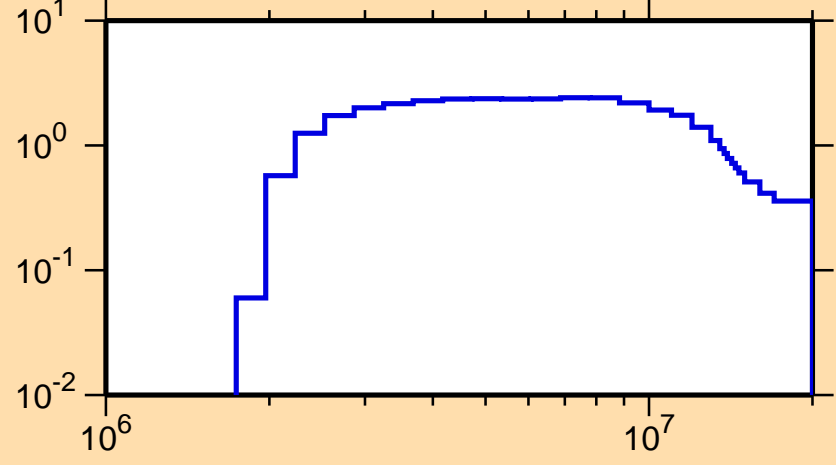
\sigma vs. E for ^{213}\text{Ra}(n,n\text{cont.})
