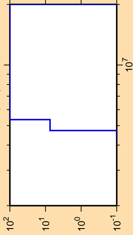
\Delta\sigma/\sigma vs. E for ^{213}\text{Ra}(n,d)
