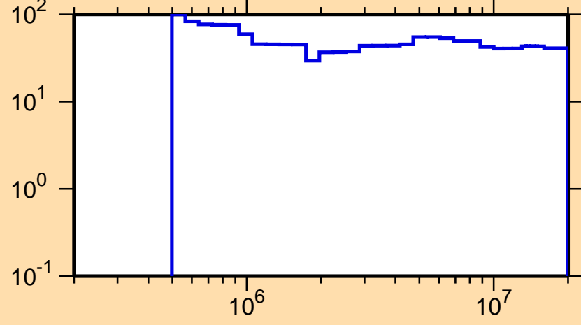
\Delta\sigma/\sigma vs. E for ^{213}\text{Ra}(n,n_1)
