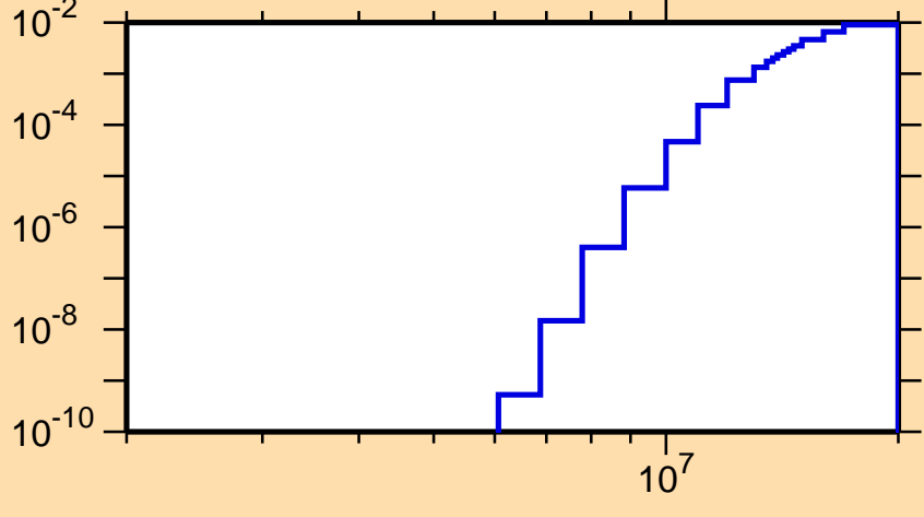
\sigma vs. E for ^{213}\text{Ra}(n,d)
