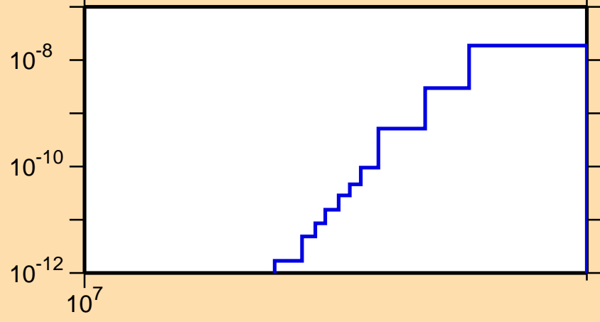
\sigma vs. E for ^{213}\text{Ra}(n,\text{pd})
