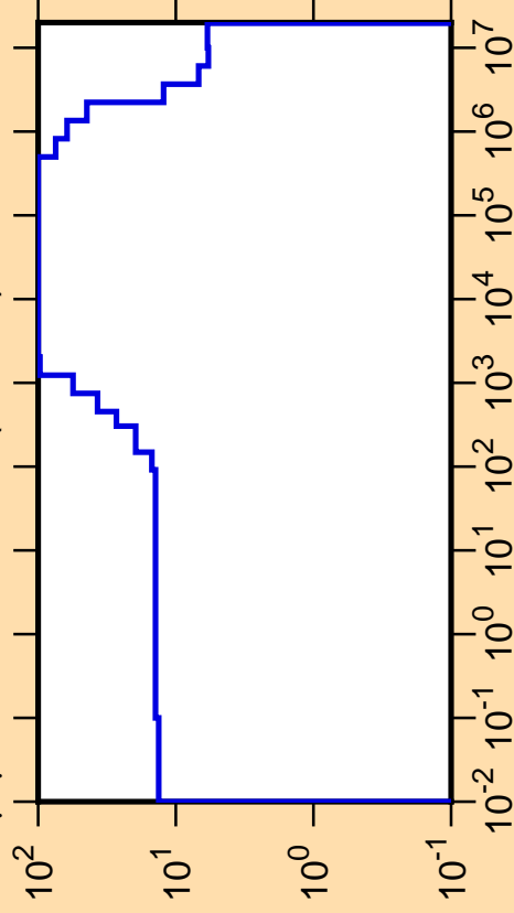
\Delta\mu/\mu vs. E for ^{213}\text{Ra}(\text{mt251})
