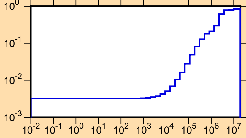
\mu vs. E for ^{213}\text{Ra}(\text{mt251})
