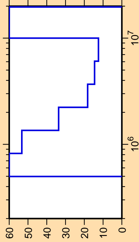
\Delta\sigma/\sigma vs. E for ^{213}\text{Ra}(n,\text{inel.})
