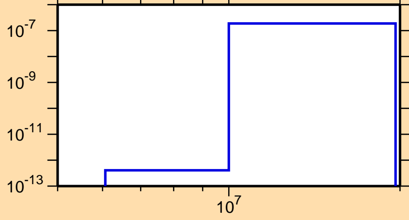
\sigma vs. E for ^{213}\text{Ra}(n,\text{He3})
