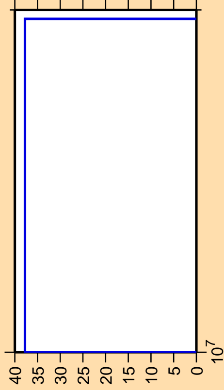
\Delta\sigma/\sigma vs. E for ^{213}\text{Ra} (mt 34)
