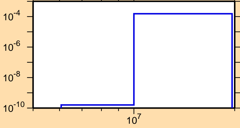
\sigma vs. E for ^{213}\text{Ra}(n,t)
