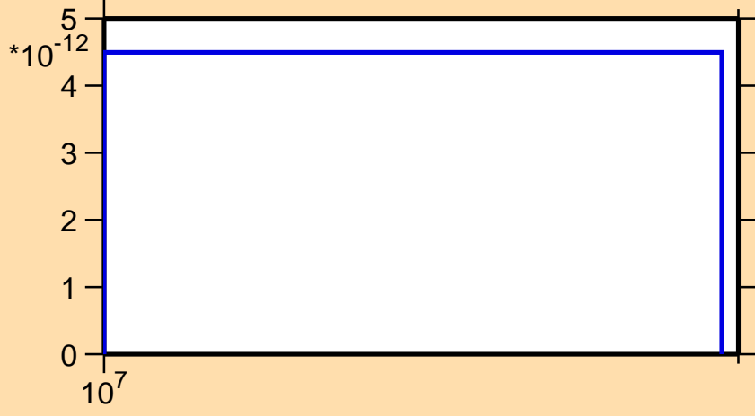
\sigma vs. E for ^{213}\text{Ra} (mt 34)
