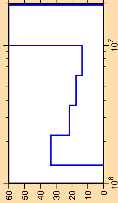
\Delta\sigma/\sigma vs. E for ^{213}\text{Ra}(n,\text{ncont.})
