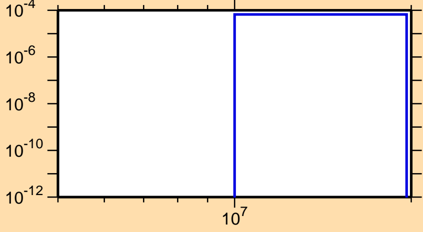
\sigma vs. E for ^{213}\text{Ra}(n,2n\alpha)
