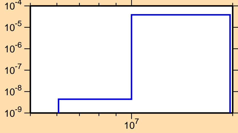
\sigma vs. E for ^{213}\text{Ra}(\text{mt } 45)
