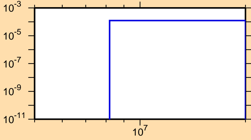
\sigma vs. E for ^{213}\text{Ra}(n,t)
