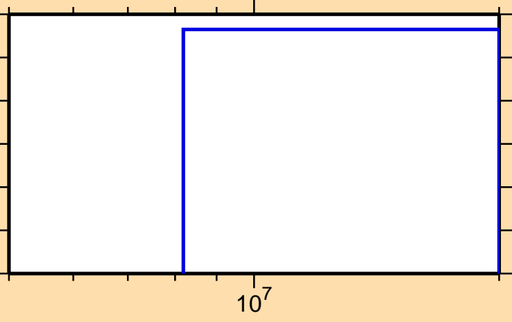
\sigma vs. E for ^{213}\text{Ra}(n,\text{pt})
