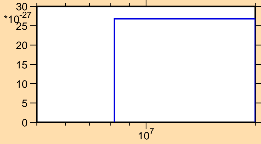
\sigma vs. E for ^{213}\text{Ra}(\text{mt } 42)
