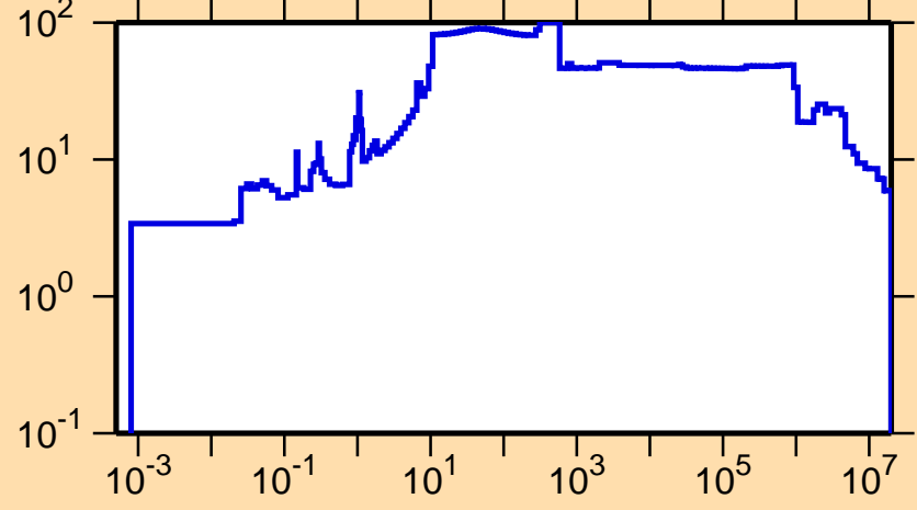
\Delta\sigma/\sigma vs. E for ^{214}\text{Ra}(n,\text{nonel.})
