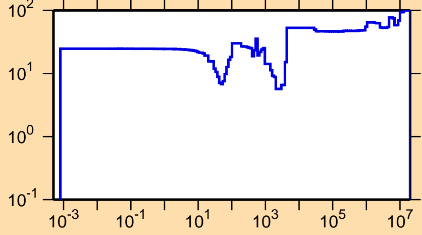
\Delta\sigma/\sigma vs. E for ^{214}\text{Ra}(n,\gamma)
