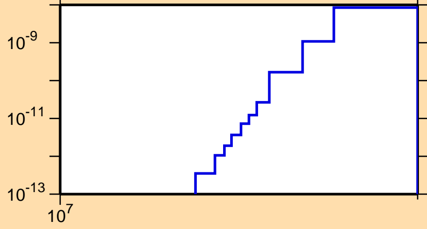
\sigma vs. E for ^{214}\text{Ra}(n,\text{pd})
