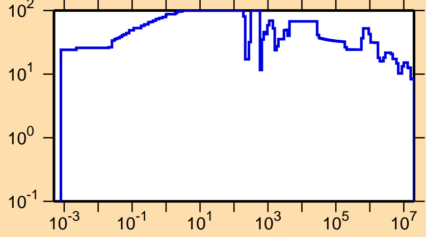
\Delta\sigma/\sigma vs. E for ^{214}\text{Ra}(n,\text{tot.})
