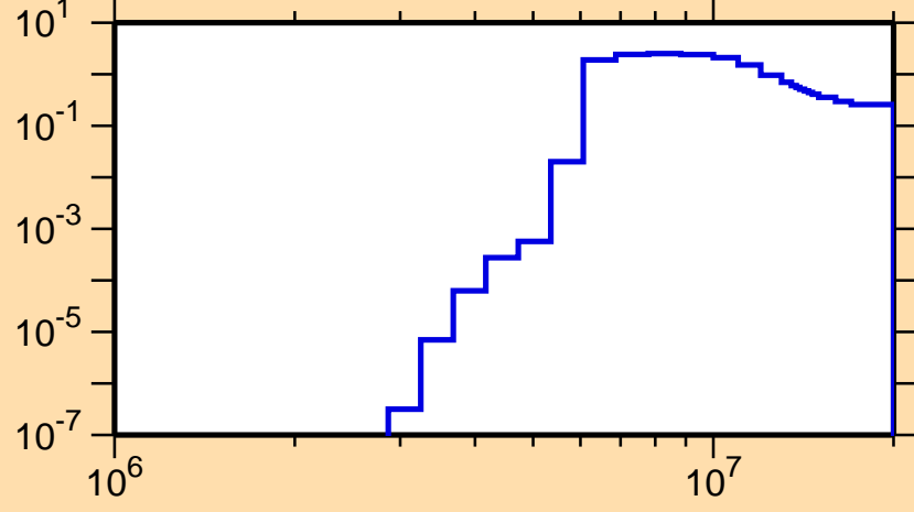
\sigma vs. E for ^{214}\text{Ra}(n,n\text{cont.})
