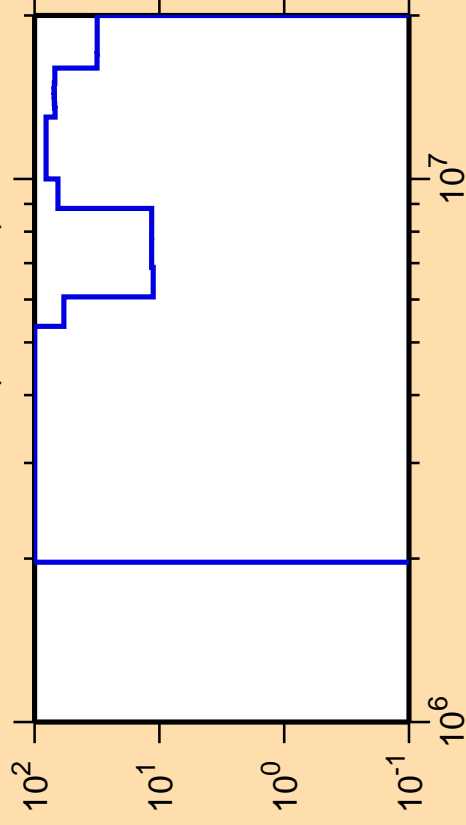
\Delta\sigma/\sigma vs. E for ^{214}\text{Ra}(n,\text{ncont.})
