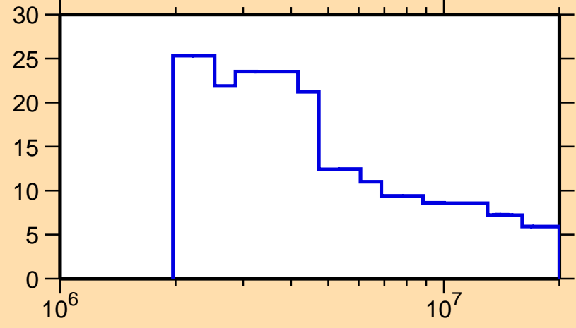
\Delta\sigma/\sigma vs. E for ^{214}\text{Ra}(n,n\text{onel.})
