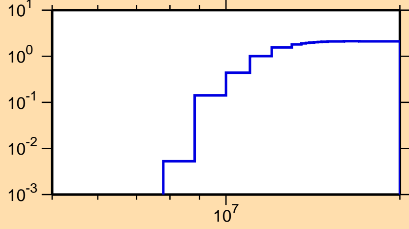
\sigma vs. E for ^{214}\text{Ra}(n,2n)
