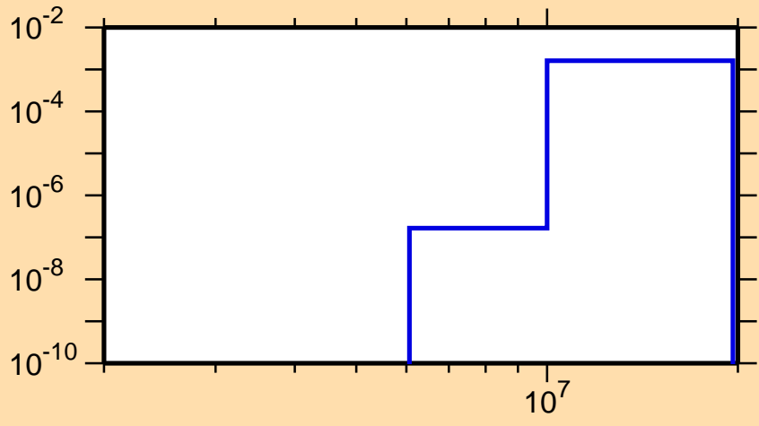
\sigma vs. E for ^{214}\text{Ra}(n,d)
