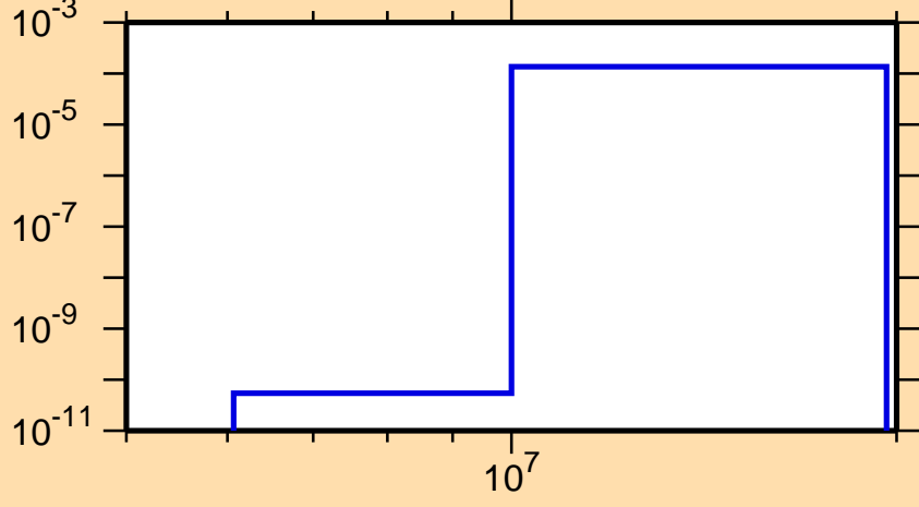
\sigma vs. E for ^{214}\text{Ra}(n,t)
