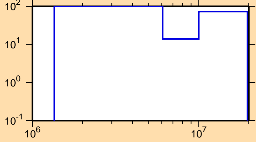
\Delta\sigma/\sigma vs. E for ^{214}\text{Ra}(n,ncont.)
