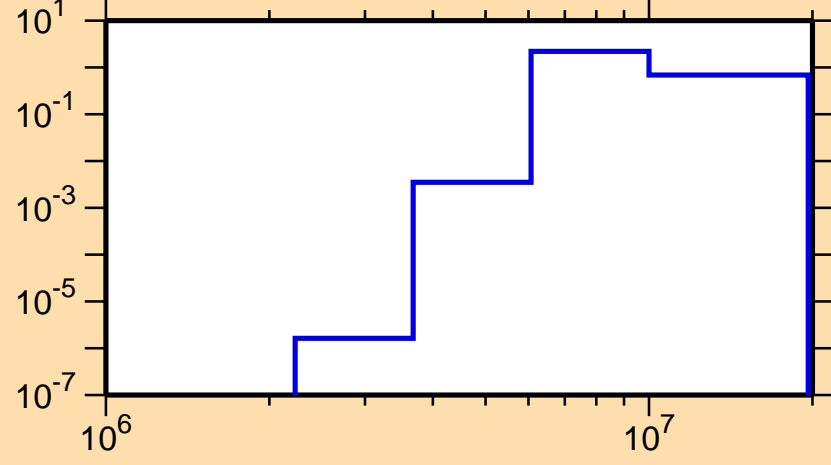
\sigma vs. E for ^{214}\text{Ra}(n,n\text{cont.})
