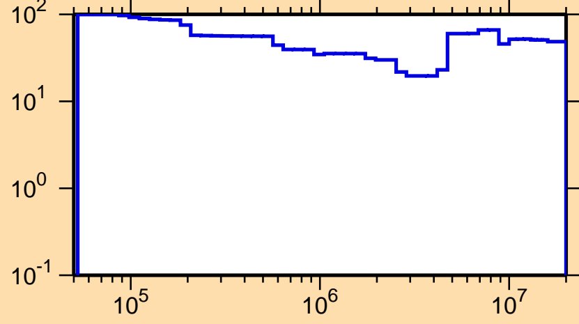
\Delta\sigma/\sigma vs. E for ^{221}\text{Ra}(n,\text{inel.})
