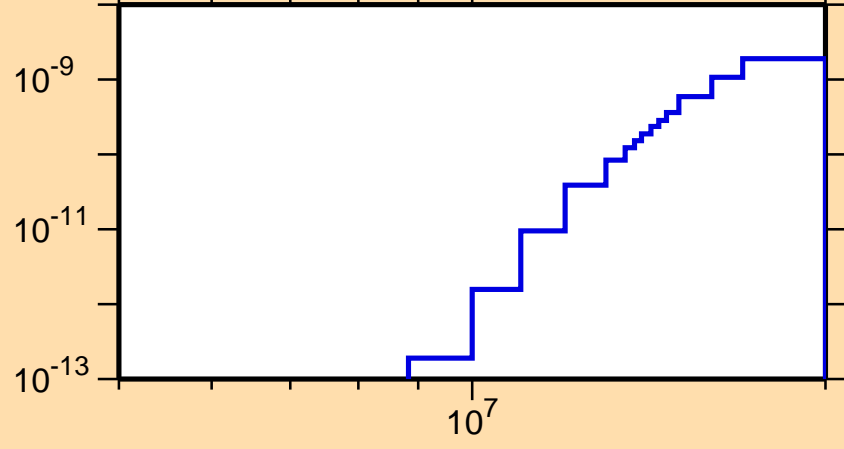
\sigma vs. E for ^{221}\text{Ra}(n,p\alpha)
