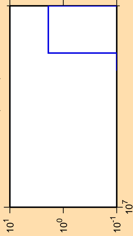
\Delta\sigma/\sigma vs. E for ^{221}\text{Ra}(\text{mt } 34)
