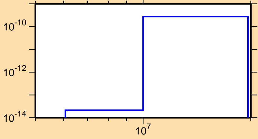
\sigma vs. E for ^{221}\text{Ra}(n,p\alpha)
