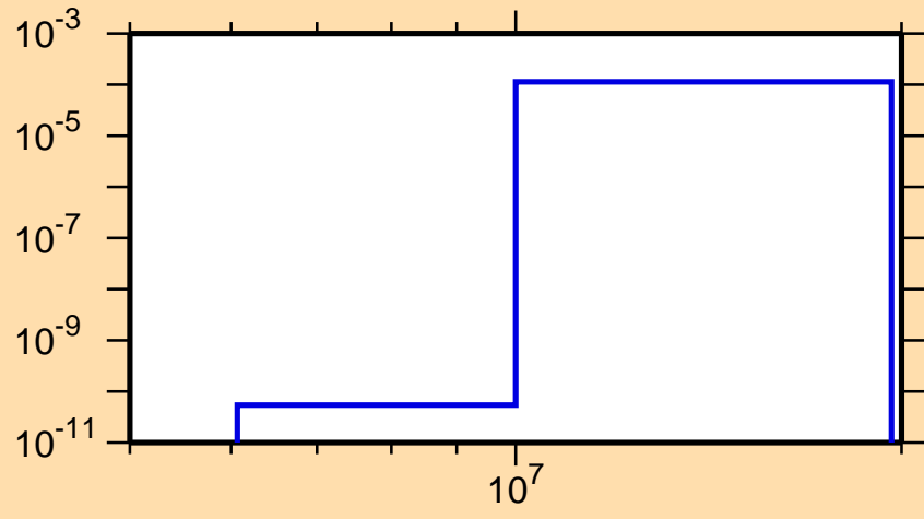
\sigma vs. E for ^{221}\text{Ra}(n,t)
