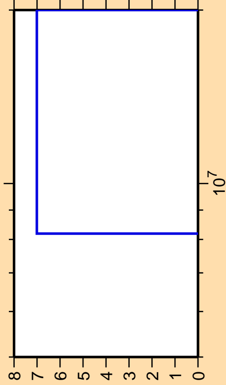
\Delta\sigma/\sigma vs. E for ^{221}\text{Ra}(\text{mt117})
