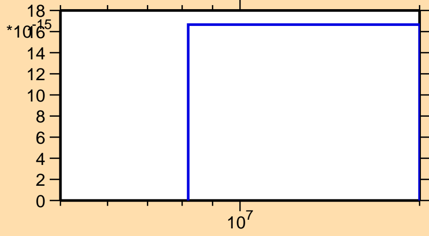
\sigma vs. E for ^{221}\text{Ra}(\text{mt } 34)
