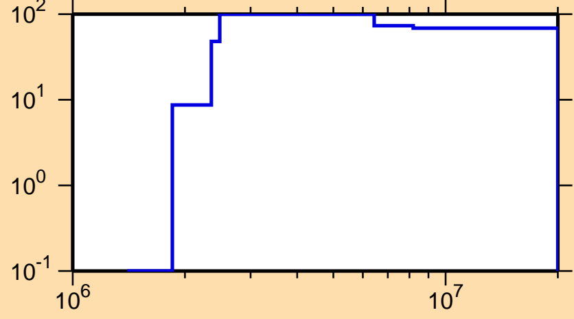
\Delta\sigma/\sigma vs. E for ^{221}\text{Ra}(n,p)
