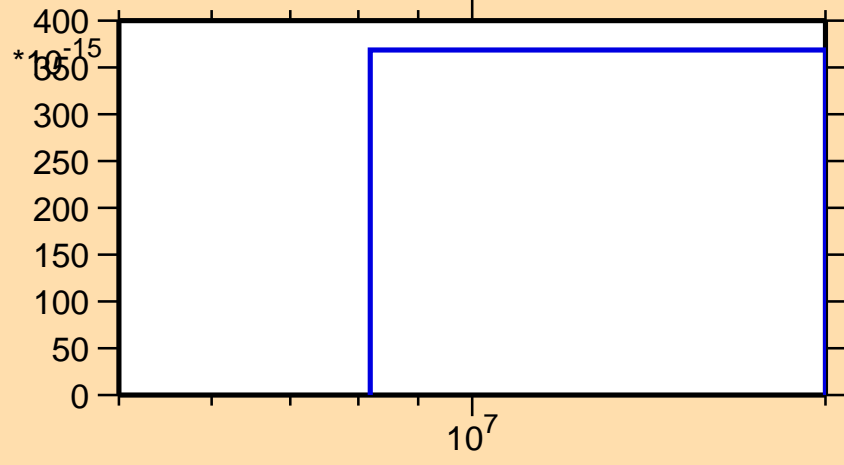
\sigma vs. E for ^{221}\text{Ra}(\text{mt } 45)
