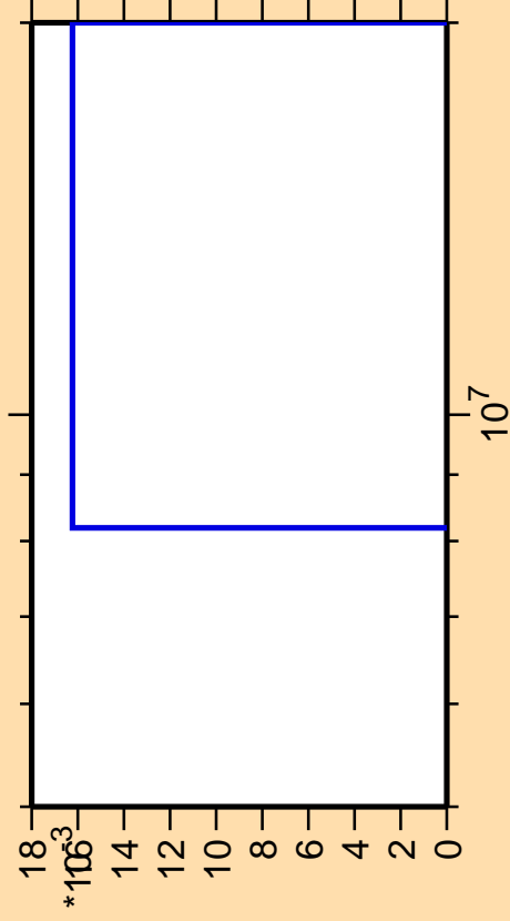
\Delta\sigma/\sigma vs. E for ^{221}\text{Ra}(\text{mt } 34)
