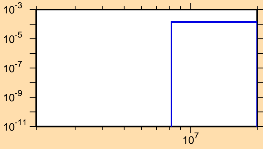
\sigma vs. E for ^{221}\text{Ra}(n,np)
