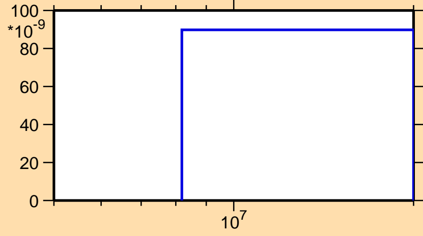
\sigma vs. E for ^{221}\text{Ra}(n,2np)
