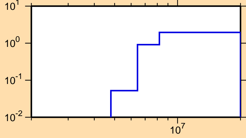
\sigma vs. E for ^{221}\text{Ra}(n,2n)
