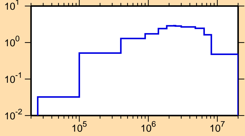
\sigma vs. E for ^{221}\text{Ra}(n,\text{inel.})
