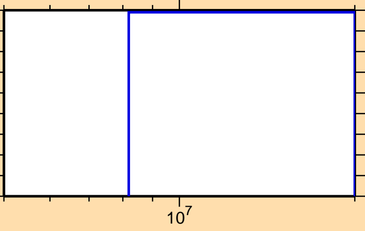
\sigma vs. E for ^{221}\text{Ra}(n,3n\alpha)
