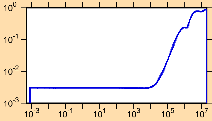
\mu vs. E for ^{222}\text{Ra}(\text{mt251})
