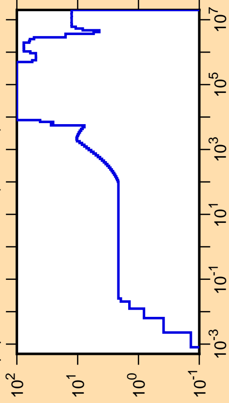
\Delta\mu/\mu vs. E for ^{222}\text{Ra}(\text{mt251})
