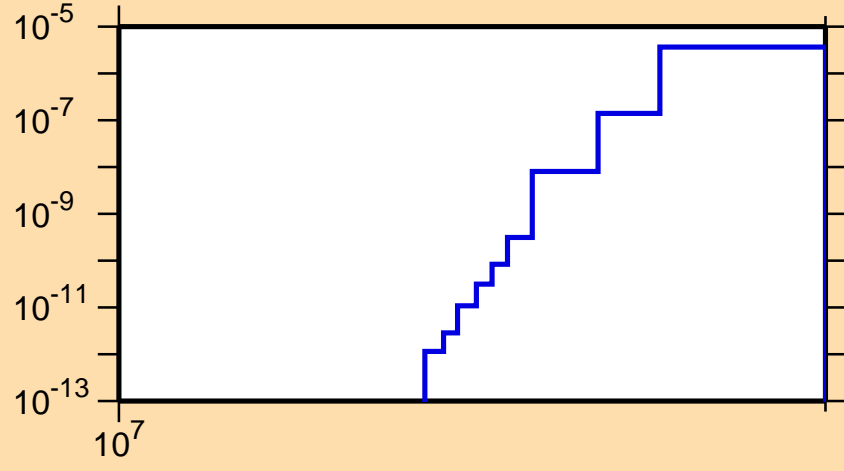
\sigma vs. E for ^{222}\text{Ra}(n,nt)
