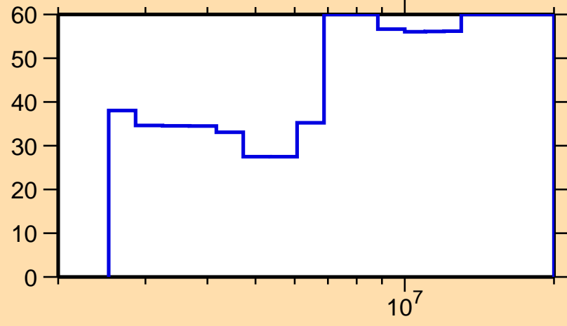
\Delta\sigma/\sigma vs. E for ^{222}\text{Ra}(n,ncont.)
