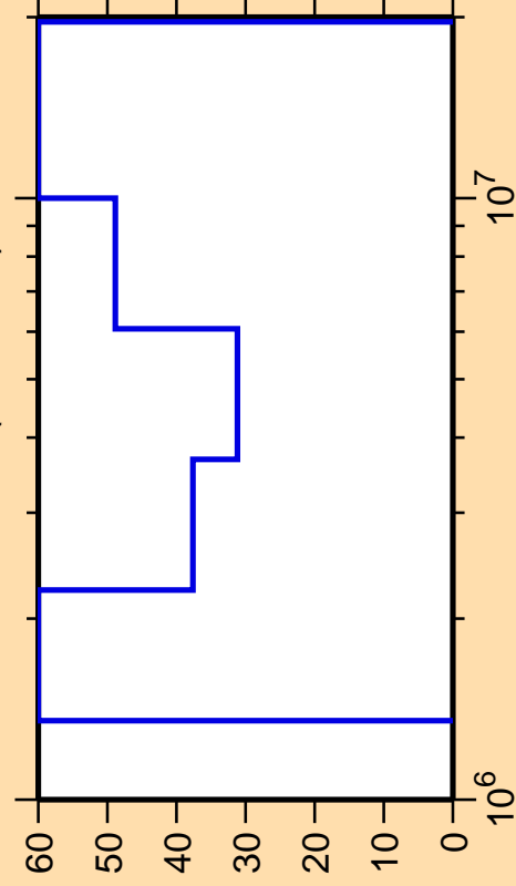
\Delta\sigma/\sigma vs. E for ^{222}\text{Ra}(n,\text{ncont.})
