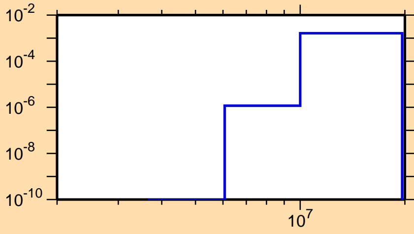
\sigma vs. E for ^{222}\text{Ra}(n,p)
