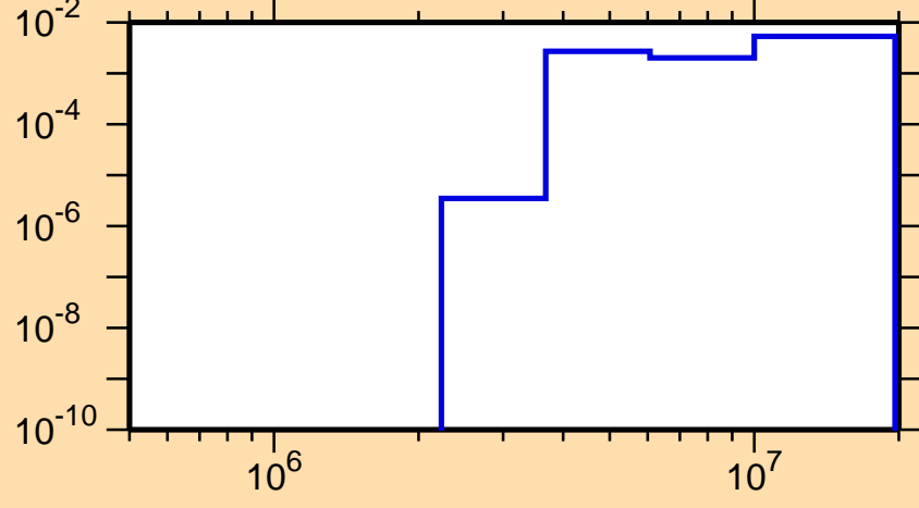
\sigma vs. E for ^{222}\text{Ra}(n,f)
