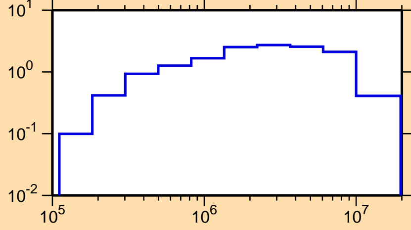
\sigma vs. E for ^{222}\text{Ra}(n,\text{inel.})
