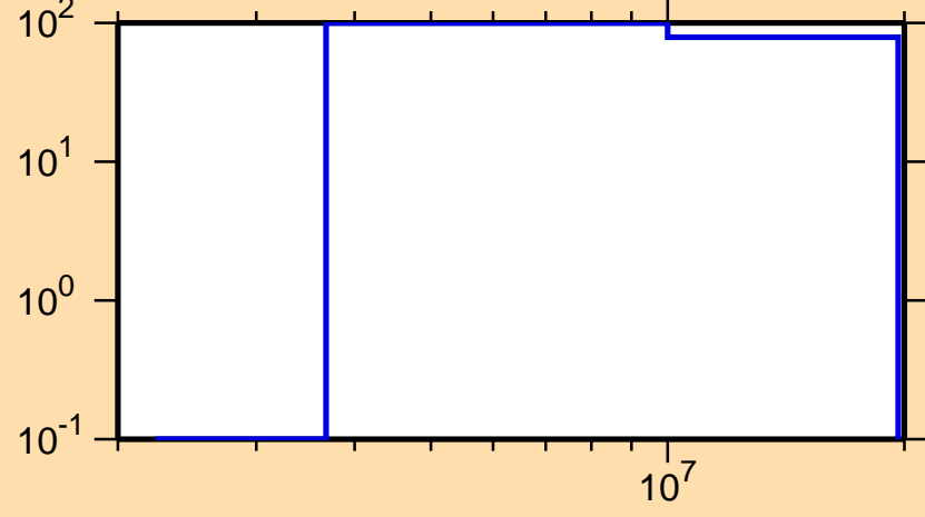
\Delta\sigma/\sigma vs. E for ^{222}\text{Ra}(n,p)
