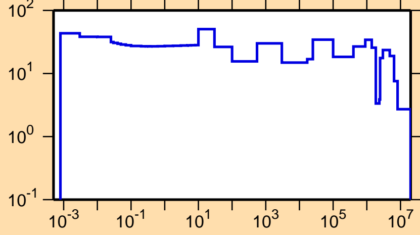
\Delta\sigma/\sigma vs. E for ^{222}\text{Ra}(n,\text{tot.})
