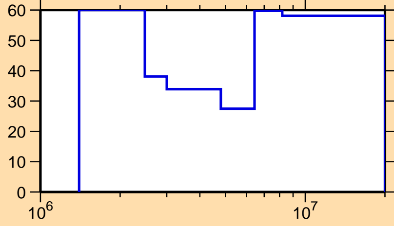
\Delta\sigma/\sigma vs. E for ^{222}\text{Ra}(n,n\text{cont.})
