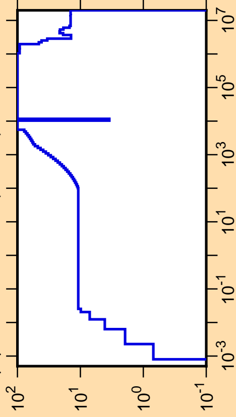
\Delta\mu/\mu vs. E for ^{223}\text{Ra}(\text{mt251})
