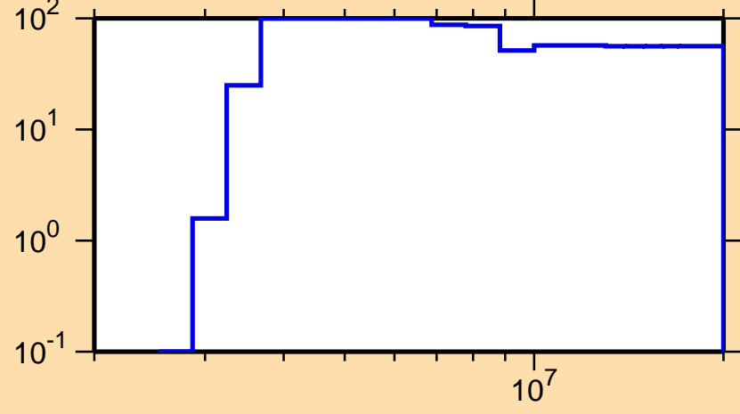
\Delta\sigma/\sigma vs. E for ^{223}\text{Ra}(n,p)
