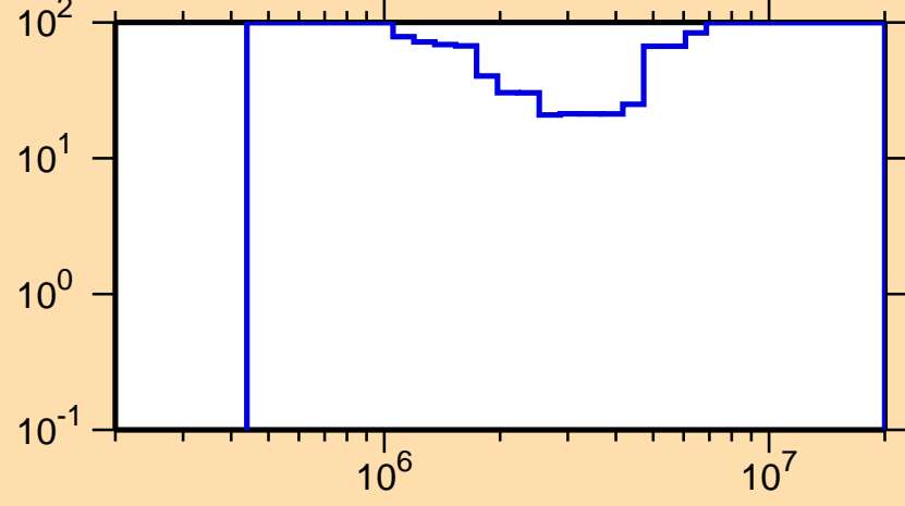
\Delta\sigma/\sigma vs. E for ^{223}\text{Ra}(n,n\text{cont.})
