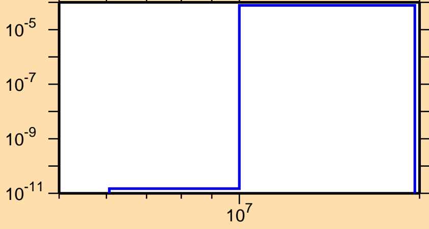
\sigma vs. E for ^{223}\text{Ra}(n,t)
