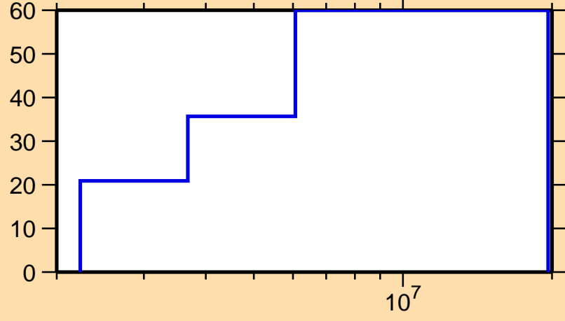
\Delta\sigma/\sigma vs. E for ^{223}\text{Ra}(n,n\text{cont.})
