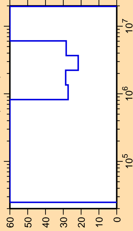
\Delta\sigma/\sigma vs. E for ^{223}\text{Ra}(n,\text{inel.})
