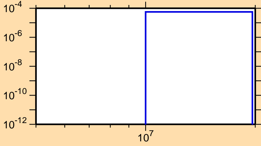
\sigma vs. E for ^{223}\text{Ra}(n,np)
