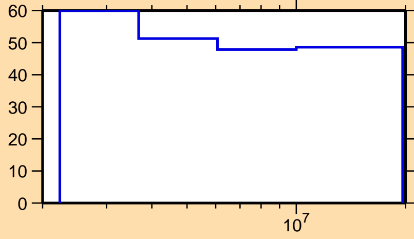
\Delta\sigma/\sigma vs. E for ^{223}\text{Ra}(n,n_1)
