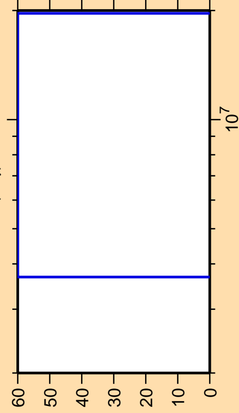
\Delta\sigma/\sigma vs. E for ^{223}\text{Ra}(n,\gamma)
