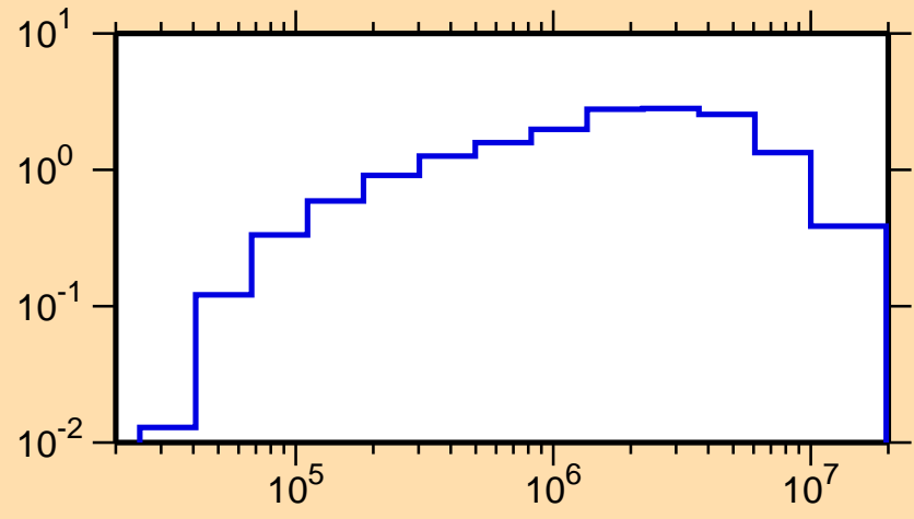
\sigma vs. E for ^{223}\text{Ra}(n,\text{inel.})
