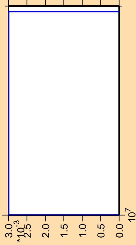
\Delta\sigma/\sigma vs. E for ^{223}\text{Ra} (mt 34)
