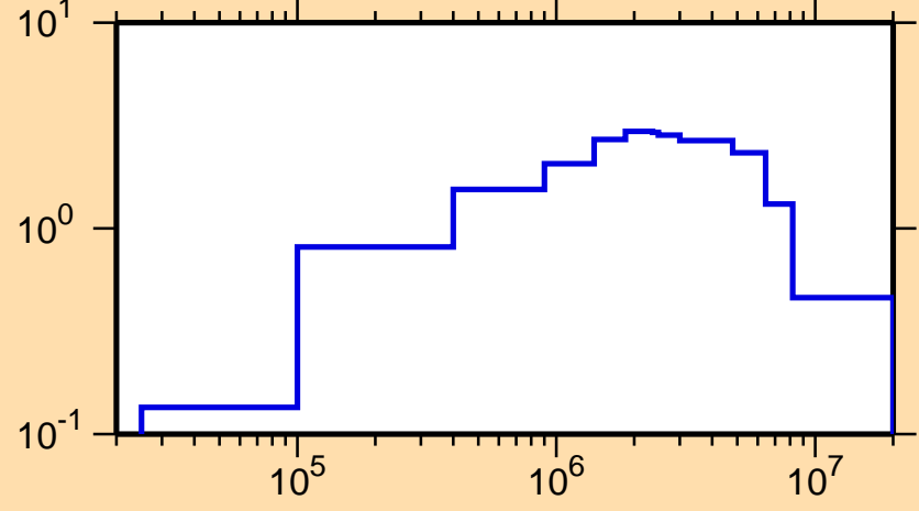
\sigma vs. E for ^{223}\text{Ra}(n,\text{inel.})
