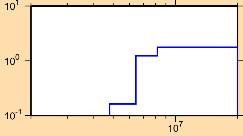
\sigma vs. E for ^{223}\text{Ra}(n,2n)
