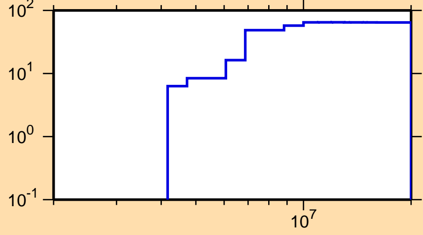
\Delta\sigma/\sigma vs. E for ^{224}\text{Ra}(n,ncont.)
