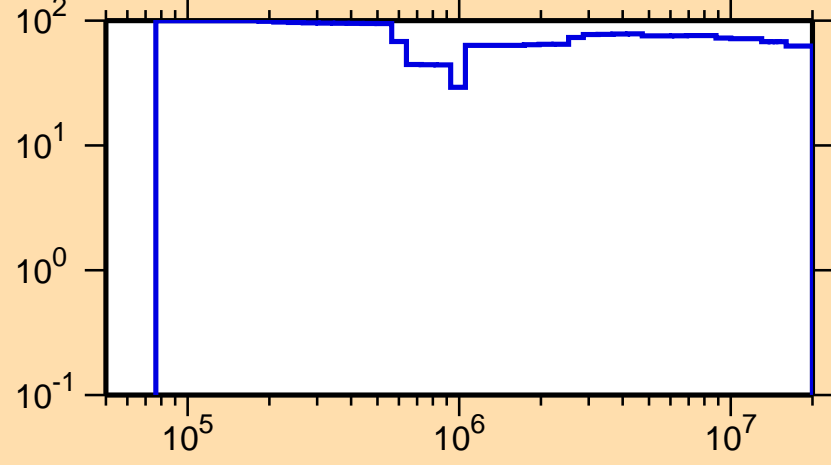
\Delta\sigma/\sigma vs. E for ^{224}\text{Ra}(n,n_1)
