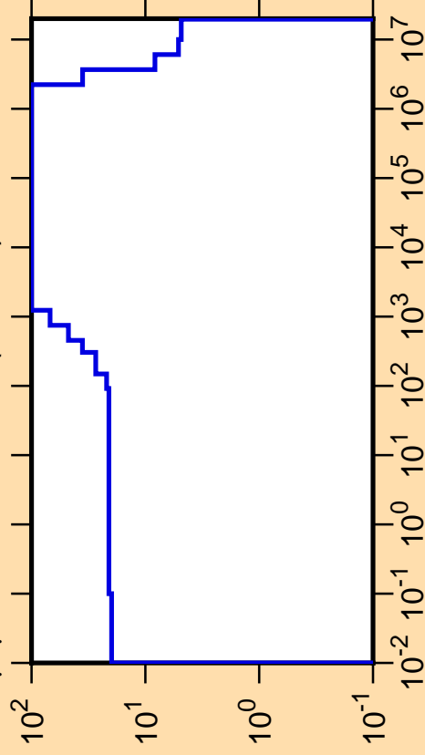
\Delta\mu/\mu vs. E for ^{224}\text{Ra}(\text{mt251})
