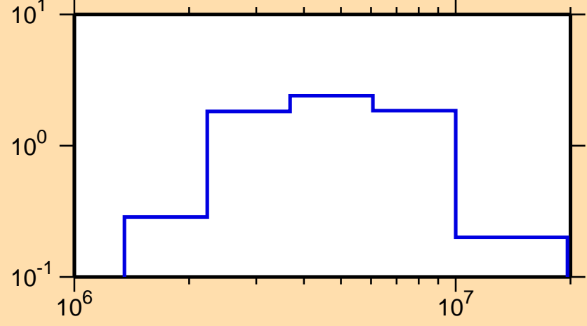
\sigma vs. E for ^{224}\text{Ra}(n,n\text{cont.})
