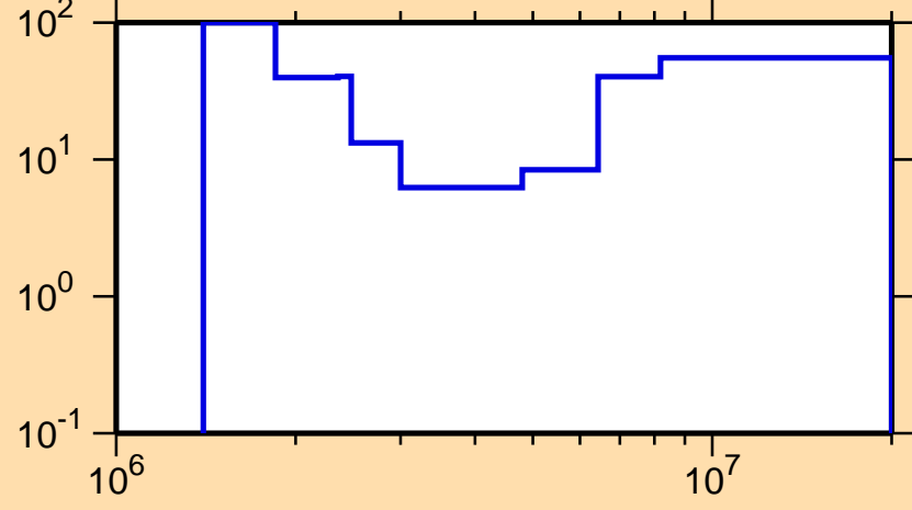
\Delta\sigma/\sigma vs. E for ^{224}\text{Ra}(n,n\text{cont.})
