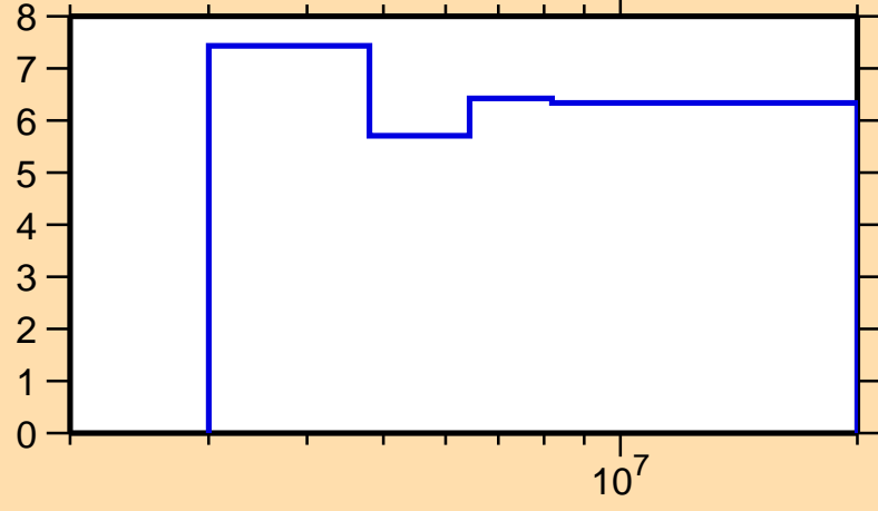
\Delta\sigma/\sigma vs. E for ^{224}\text{Ra}(n,\text{nonel.})
