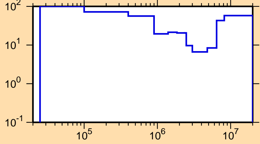
\Delta\sigma/\sigma vs. E for ^{224}\text{Ra}(n,\text{inel.})
