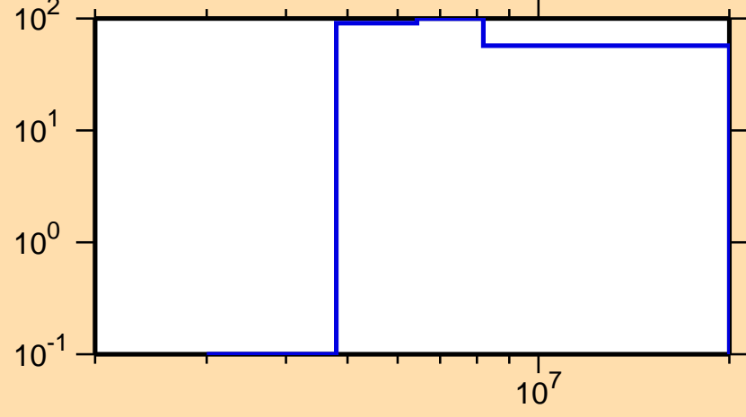
\Delta\sigma/\sigma vs. E for ^{224}\text{Ra}(n,p)
