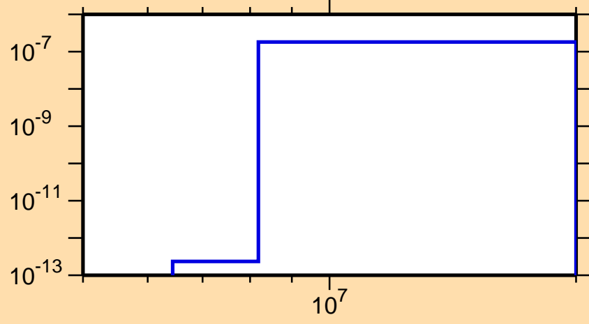
\sigma vs. E for ^{224}\text{Ra}(n,2n\alpha)
