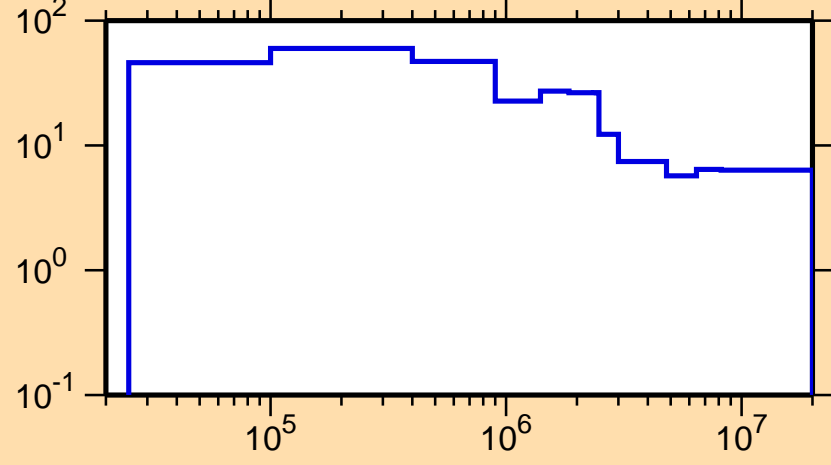
\Delta\sigma/\sigma vs. E for ^{224}\text{Ra}(n,\text{nonel.})
