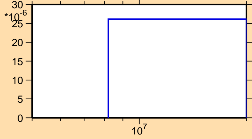
\sigma vs. E for ^{224}\text{Ra}(n,t)
