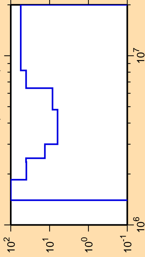
\Delta\sigma/\sigma vs. E for ^{224}\text{Ra}(n,\text{ncont.})
