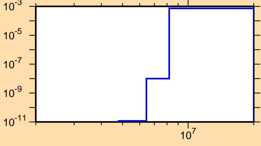
\sigma vs. E for ^{224}\text{Ra}(n,p)
