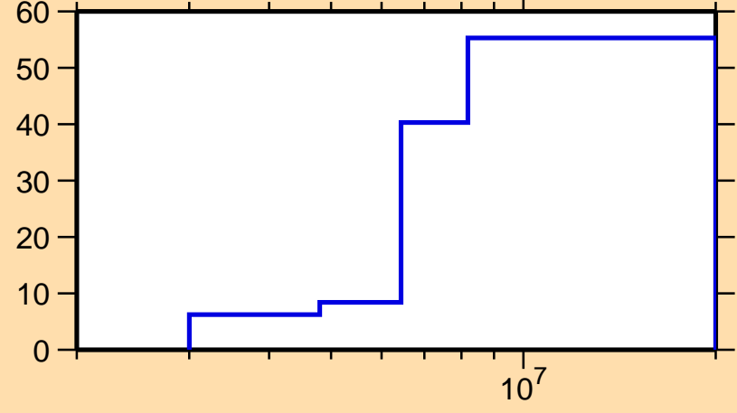
\Delta\sigma/\sigma vs. E for ^{224}\text{Ra}(n,n\text{cont.})
