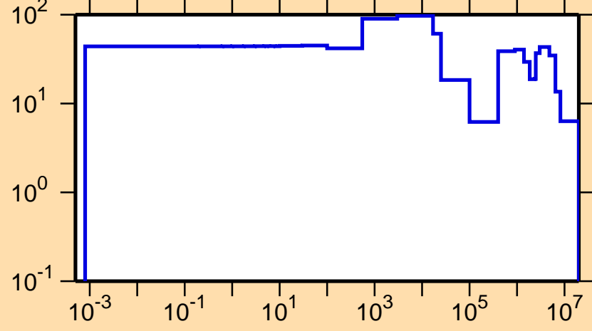
\Delta\sigma/\sigma vs. E for ^{224}\text{Ra}(n,\text{el.})
