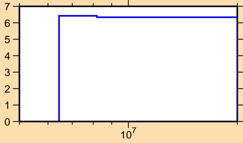
\Delta\sigma/\sigma vs. E for ^{224}\text{Ra}(n,\text{nonel.})
