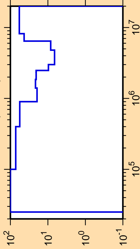
\Delta\sigma/\sigma vs. E for ^{224}\text{Ra}(n,\text{inel.})
