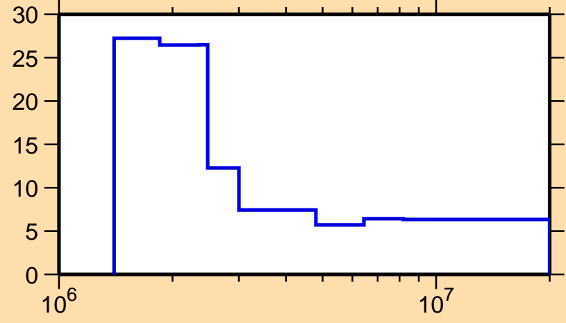
\Delta\sigma/\sigma vs. E for ^{224}\text{Ra}(n,n\text{onel.})
