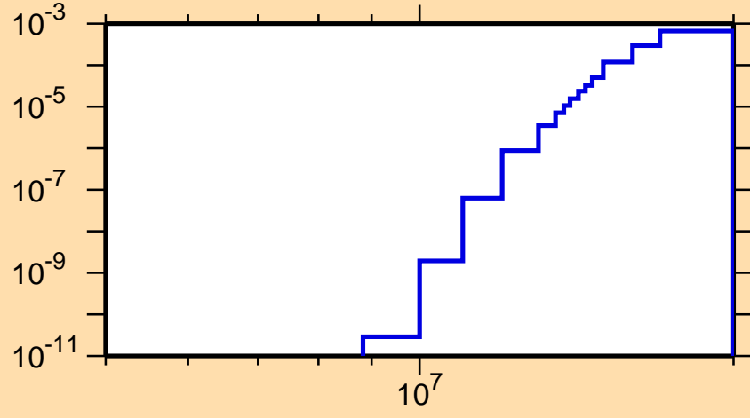
\sigma vs. E for ^{225}\text{Ra}(n,t)
