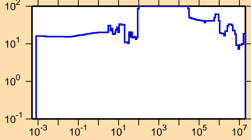
\Delta\sigma/\sigma vs. E for ^{225}\text{Ra}(n,\text{tot.})
