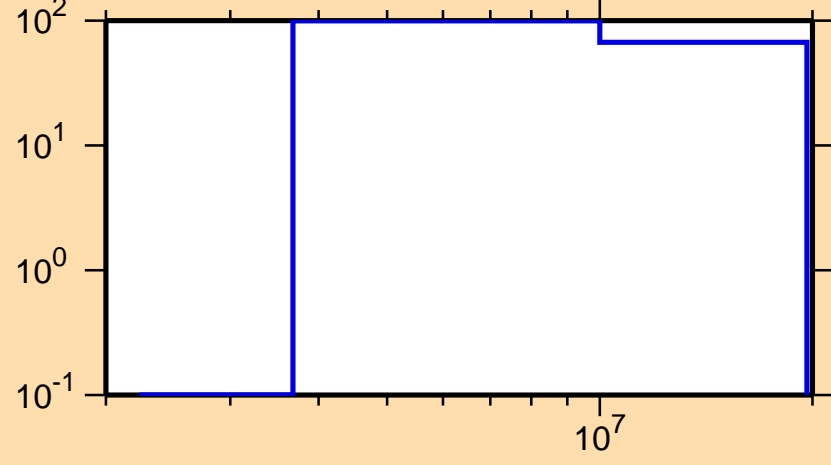
\Delta\sigma/\sigma vs. E for ^{225}\text{Ra}(n,p)
