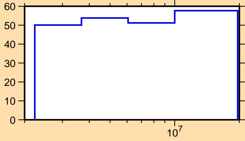
\Delta\sigma/\sigma vs. E for ^{225}\text{Ra}(n,n_1)
