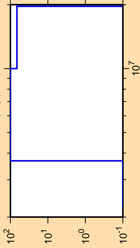
\Delta\sigma/\sigma vs. E for ^{225}\text{Ra}(n,p)
