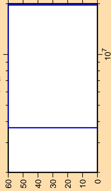
\Delta\sigma/\sigma vs. E for ^{225}\text{Ra}(n,\gamma)
