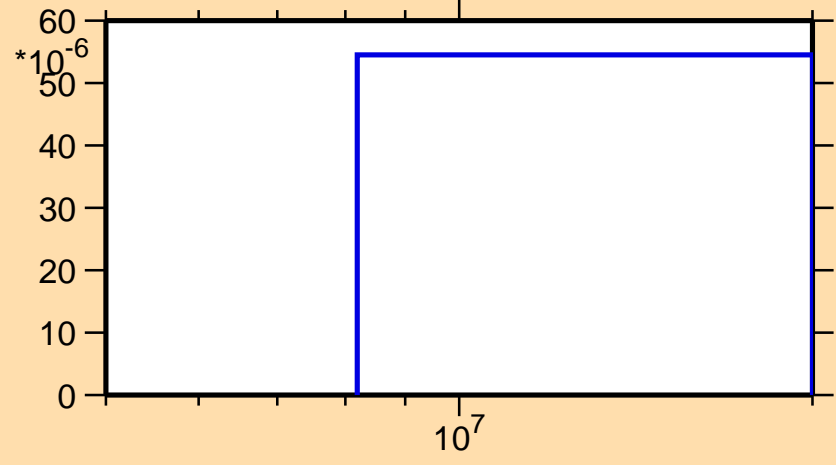
\sigma vs. E for ^{225}\text{Ra}(n,d)
