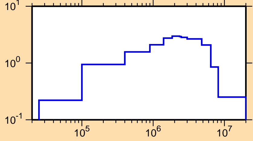
\sigma vs. E for ^{225}\text{Ra}(n,\text{inel.})
