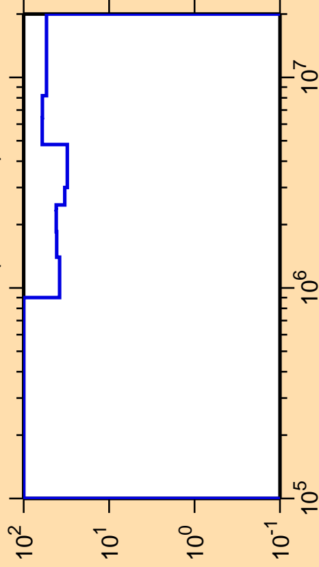
\Delta\sigma/\sigma vs. E for ^{225}\text{Ra}(n,\text{ncont.})
