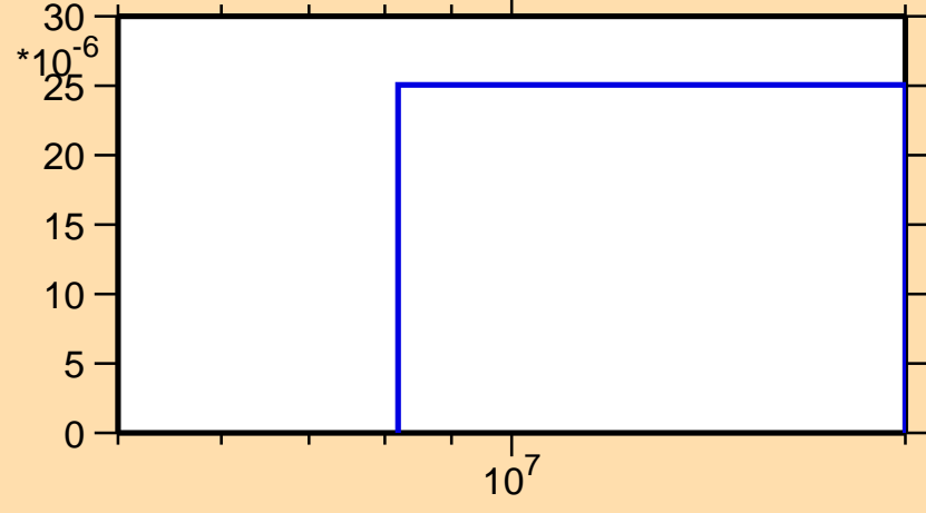
\sigma vs. E for ^{225}\text{Ra}(n,np)
