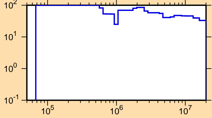
\Delta\sigma/\sigma vs. E for ^{226}\text{Ra}(n,n_1)
