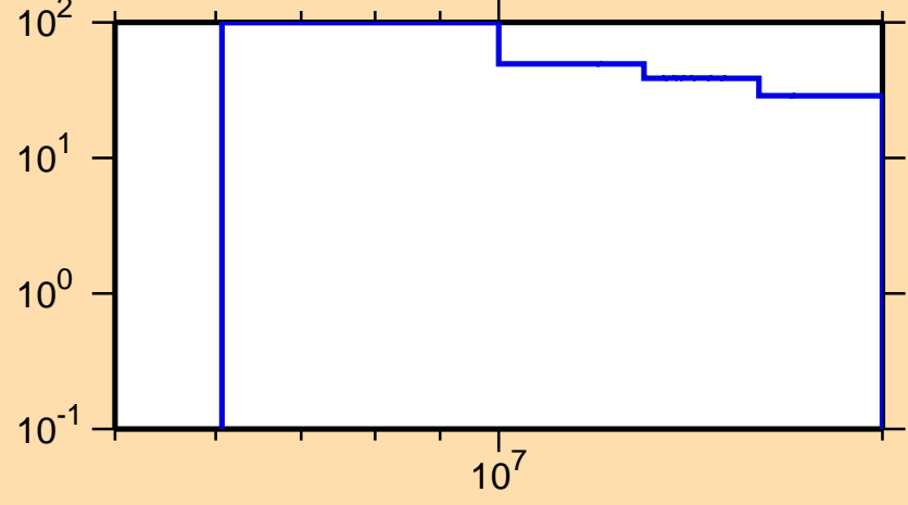
\Delta\sigma/\sigma vs. E for ^{226}\text{Ra}(n,f)
