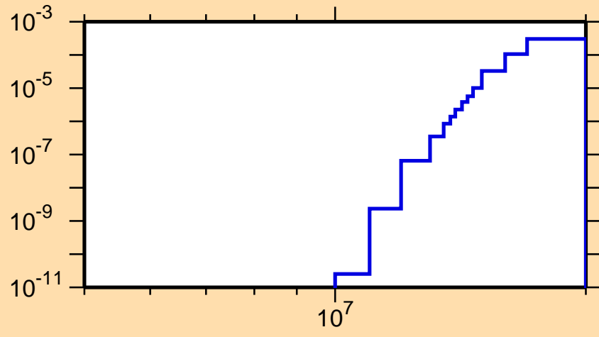
\sigma vs. E for ^{226}\text{Ra}(n,t)
