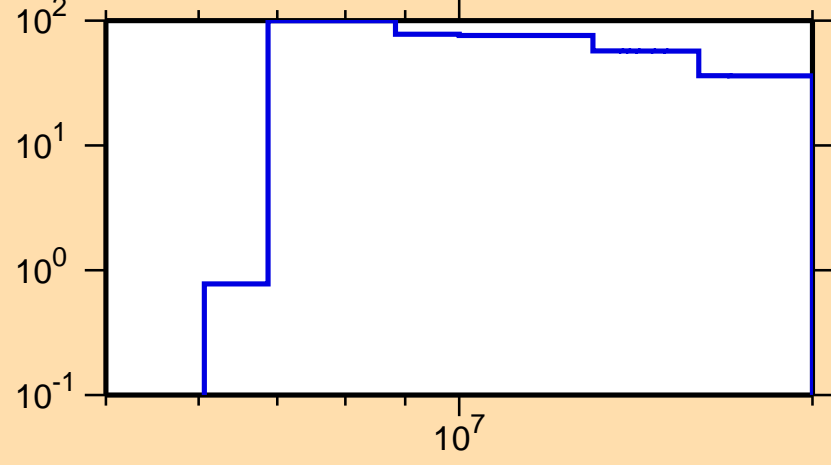
\Delta\sigma/\sigma vs. E for ^{226}\text{Ra}(n,p)
