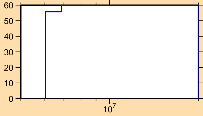
\Delta\sigma/\sigma vs. E for ^{226}\text{Ra}(n,ncont.)
