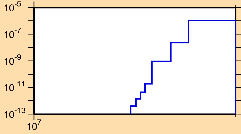
\sigma vs. E for ^{226}\text{Ra}(n,nt)
