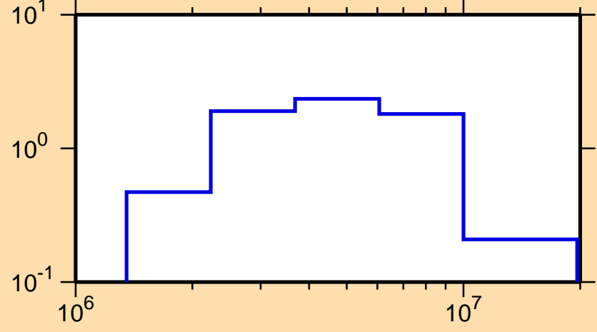
\sigma vs. E for ^{226}\text{Ra}(n,n\text{cont.})
