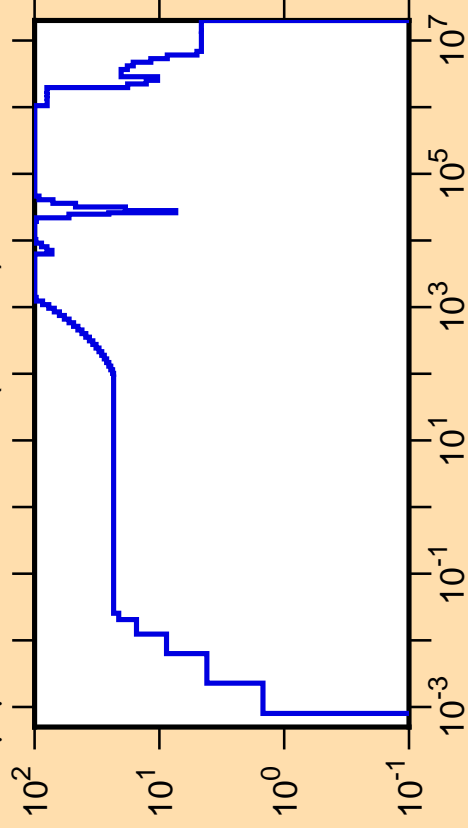
\Delta\mu/\mu vs. E for ^{227}\text{Ra}(\text{mt251})
