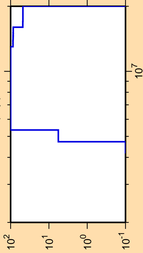
\Delta\sigma/\sigma vs. E for ^{227}\text{Ra}(n,p)
