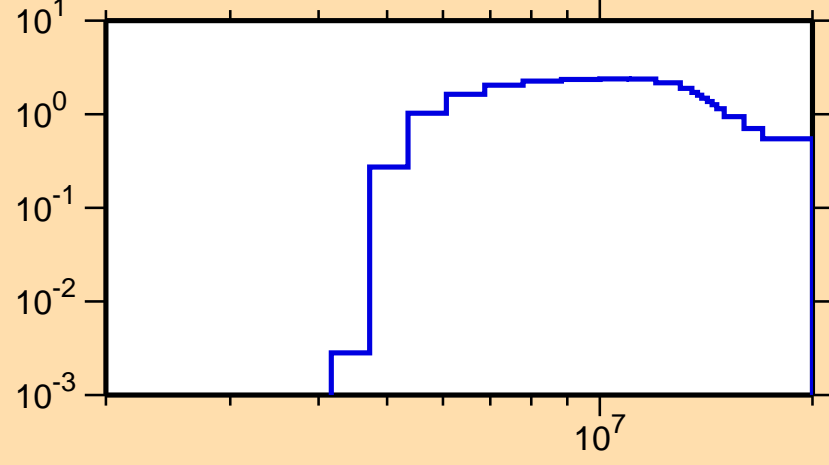
\sigma vs. E for ^{227}\text{Ra}(n,2n)
