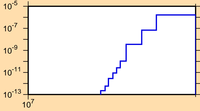
\sigma vs. E for ^{227}\text{Ra}(n,\text{nd})
