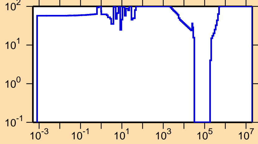
\Delta\sigma/\sigma vs. E for ^{227}\text{Ra}(n,f)
