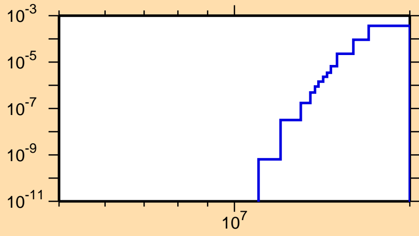
\sigma vs. E for ^{227}\text{Ra}(n,np)
