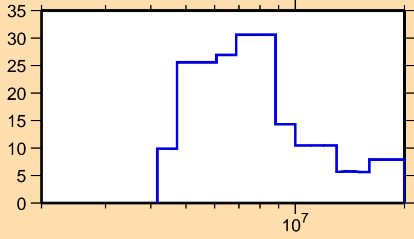
\Delta\sigma/\sigma vs. E for ^{227}\text{Ra}(n,el.)
