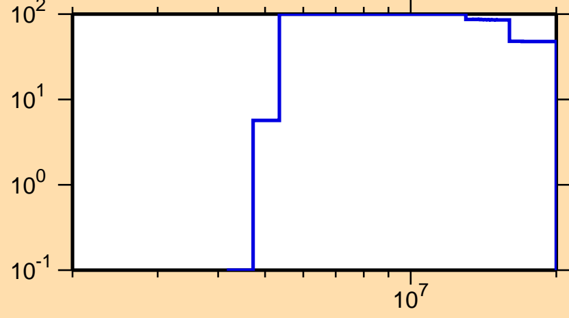
\Delta\sigma/\sigma vs. E for ^{227}\text{Ra}(n,p)
