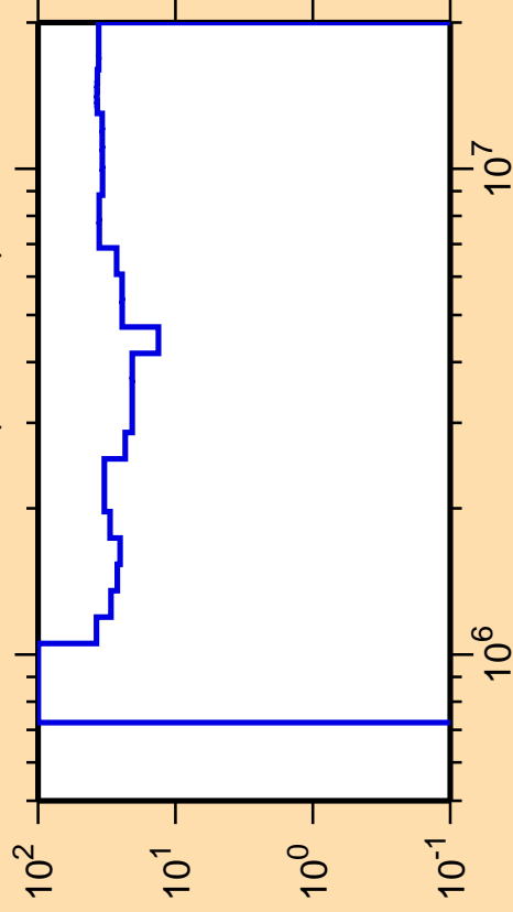
\Delta\sigma/\sigma vs. E for ^{227}\text{Ra}(n,\text{ncont.})
