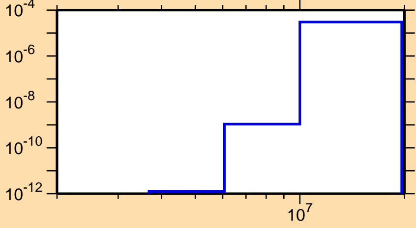
\sigma vs. E for ^{227}\text{Ra}(n,\alpha)
