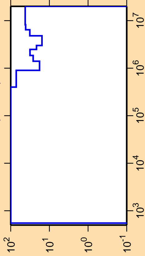
\Delta\sigma/\sigma vs. E for ^{227}\text{Ra}(n,\text{inel.})
