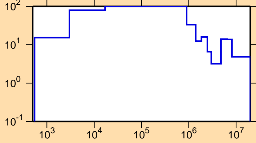
\Delta\sigma/\sigma vs. E for ^{227}\text{Ra}(n,\text{tot.})
