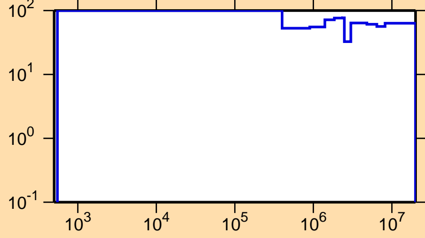
\Delta\sigma/\sigma vs. E for ^{227}\text{Ra}(n,n_1)
