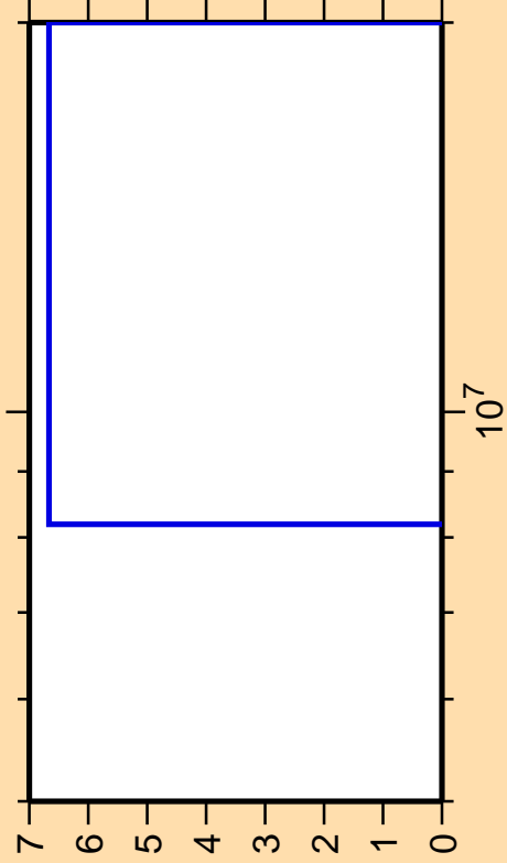
\Delta\sigma/\sigma vs. E for ^{227}\text{Ra}(n,3n\alpha)
