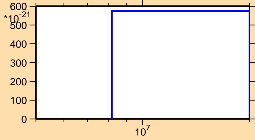
\sigma vs. E for ^{227}\text{Ra}(\text{mt } 42)
