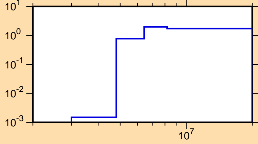
\sigma vs. E for ^{227}\text{Ra}(n,2n)
