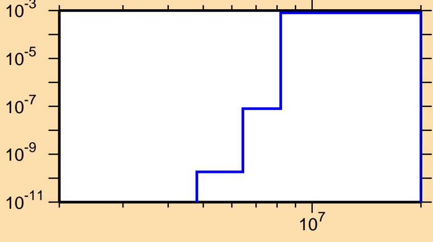
\sigma vs. E for ^{227}\text{Ra}(n,p)
