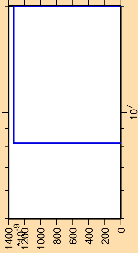
\Delta\sigma/\sigma vs. E for ^{227}\text{Ra}(\text{mt } 42)
