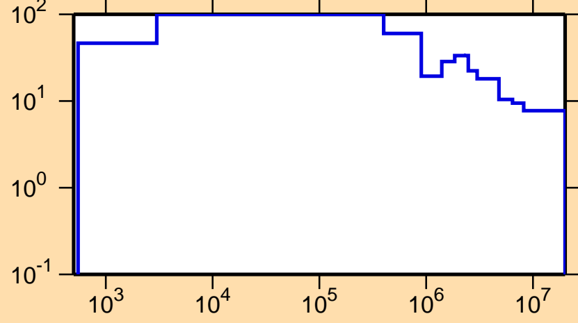
\Delta\sigma/\sigma vs. E for ^{227}\text{Ra}(n,\text{nonel.})
