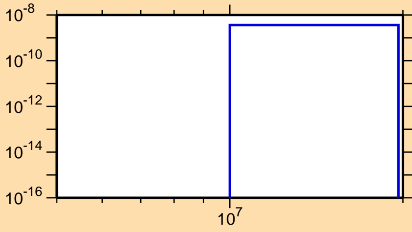
\sigma vs. E for ^{228}\text{Ra}(n,2n\alpha)
