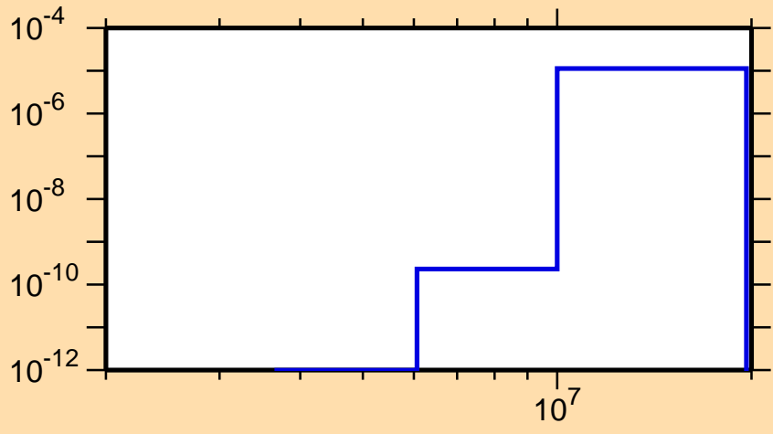
\sigma vs. E for ^{228}\text{Ra}(n,\alpha)
