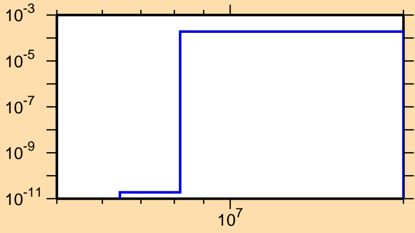
\sigma vs. E for ^{228}\text{Ra}(n,p)
