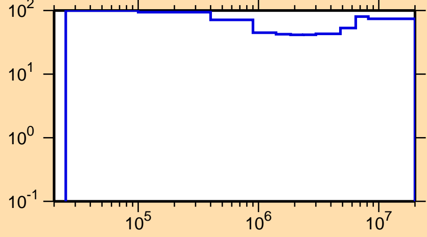
\Delta\sigma/\sigma vs. E for ^{228}\text{Ra}(n,\text{inel.})
