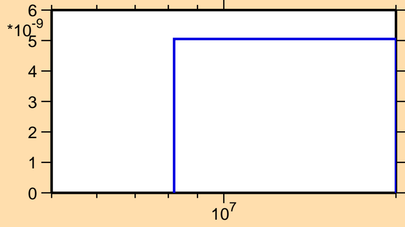
\sigma vs. E for ^{228}\text{Ra}(n,nt)
