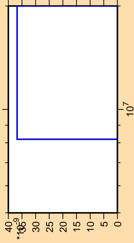
\Delta\sigma/\sigma vs. E for ^{228}\text{Ra} (mt 42)
