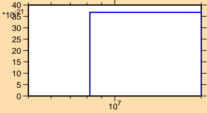
\sigma vs. E for ^{228}\text{Ra} (mt 42)
