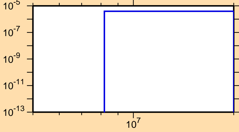
\sigma vs. E for ^{228}\text{Ra}(n,np)
