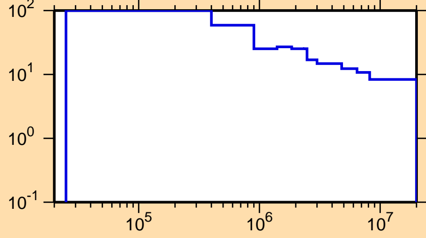
\Delta\sigma/\sigma vs. E for ^{228}\text{Ra}(n,\text{nonel.})
