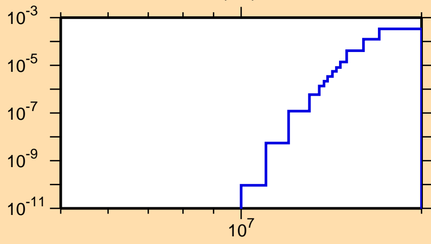
\sigma vs. E for ^{229}\text{Ra}(n,t)
