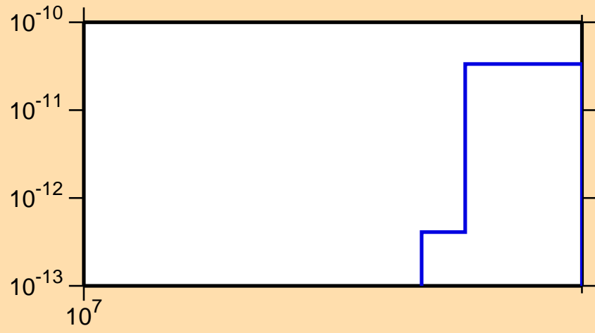
\sigma vs. E for ^{229}\text{Ra}(n,3n\alpha)
