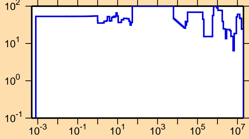
\Delta\sigma/\sigma vs. E for ^{229}\text{Ra}(n, \text{el.})
