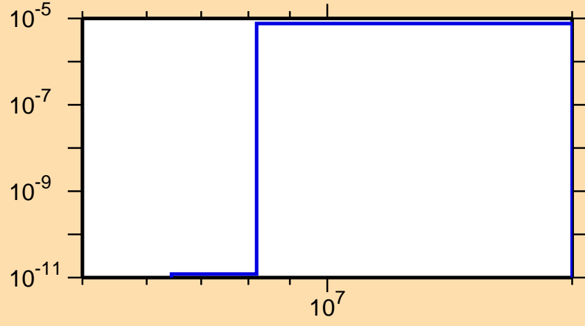
\sigma vs. E for ^{229}\text{Ra}(n,\alpha)
