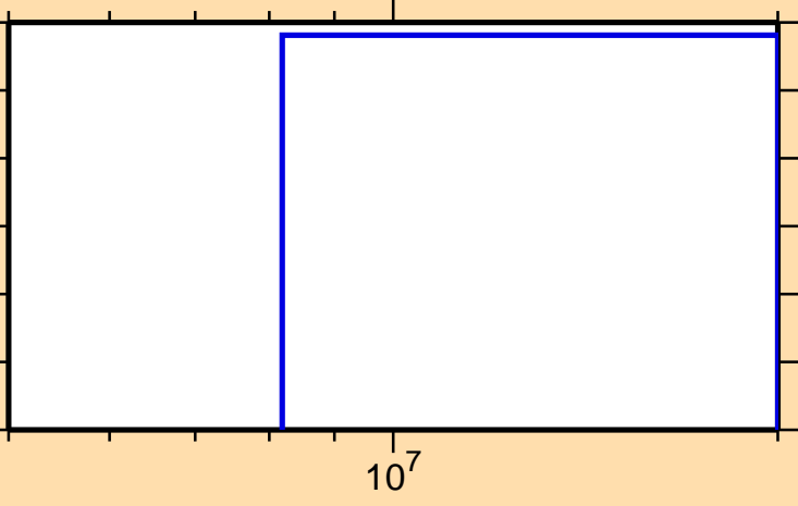
\sigma vs. E for ^{229}\text{Ra}(n,3n\alpha)
