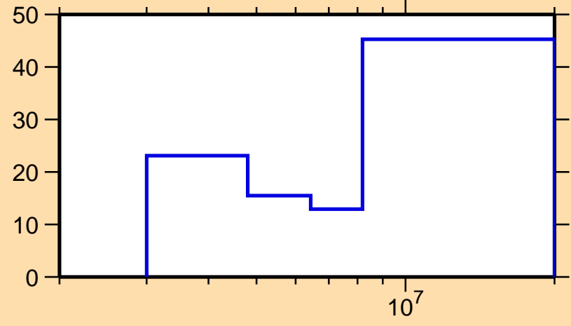
\Delta\sigma/\sigma vs. E for ^{229}\text{Ra}(n,el.)
