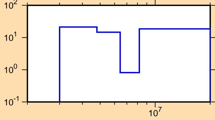
\Delta\sigma/\sigma vs. E for ^{229}\text{Ra}(n,\text{tot.})
