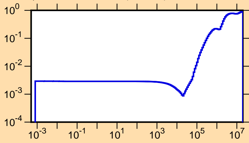
\mu vs. E for ^{230}\text{Ra}(\text{mt251})
