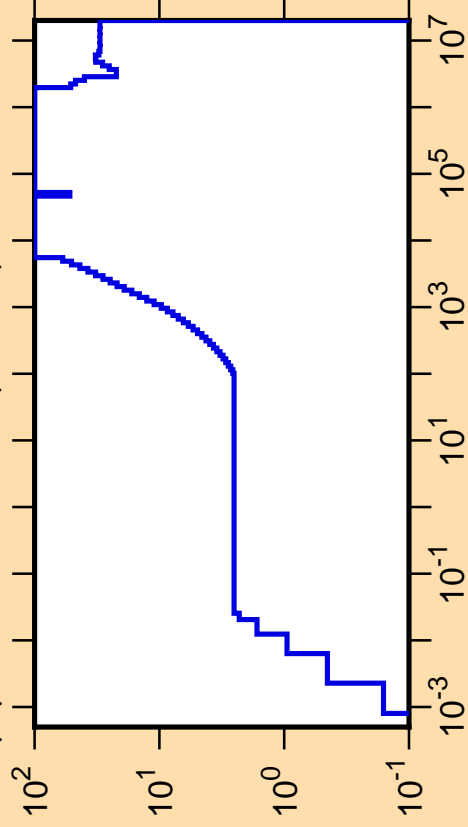
\Delta\mu/\mu vs. E for ^{230}\text{Ra}(\text{mt251})
