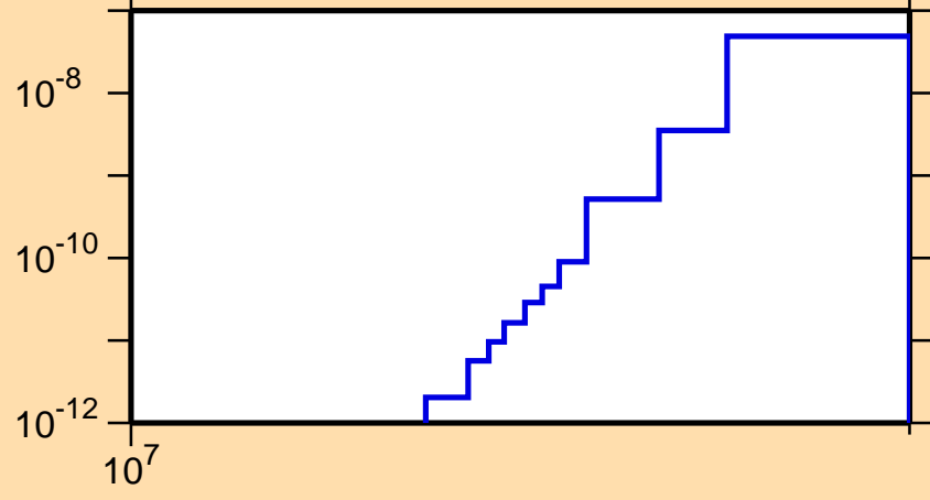
\sigma vs. E for ^{230}\text{Ra}(n,2n\alpha)
