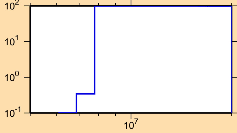
\Delta\sigma/\sigma vs. E for ^{230}\text{Ra}(n,p)
