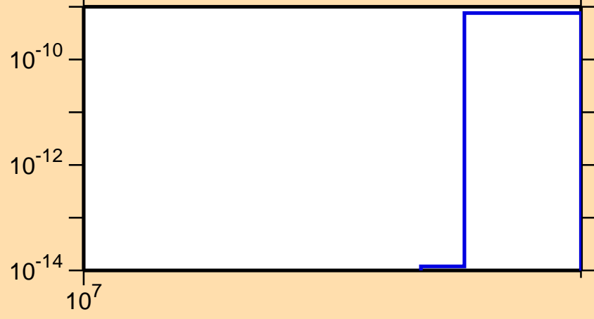
\sigma vs. E for ^{230}\text{Ra}(n,2np)
