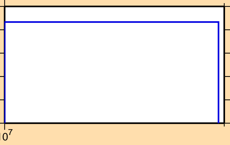
\sigma vs. E for ^{230}\text{Ra}(n,nt)
