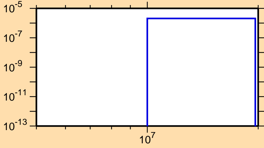
\sigma vs. E for ^{230}\text{Ra}(n,np)
