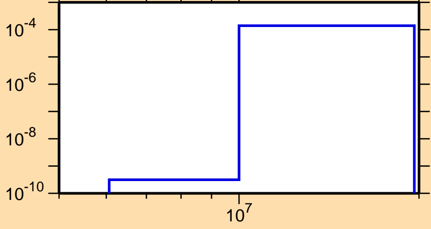
\sigma vs. E for ^{230}\text{Ra}(n,p)
