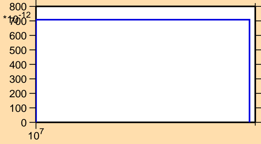
\sigma vs. E for ^{230}\text{Ra}(n,2n\alpha)
