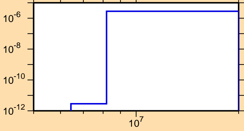
\sigma vs. E for ^{230}\text{Ra}(n,n\alpha)
