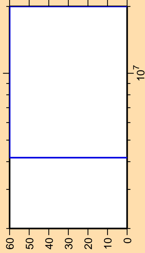
\Delta\sigma/\sigma vs. E for ^{231}\text{Ra}(n,2n)
