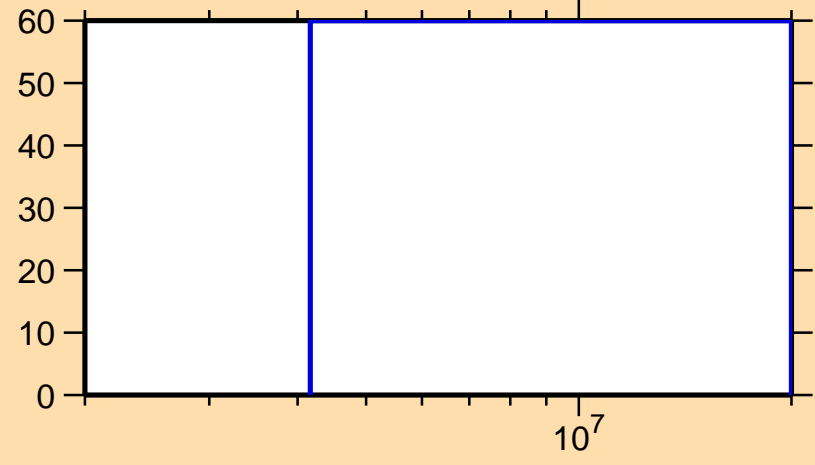
\Delta\sigma/\sigma vs. E for ^{231}\text{Ra}(n,\gamma)
