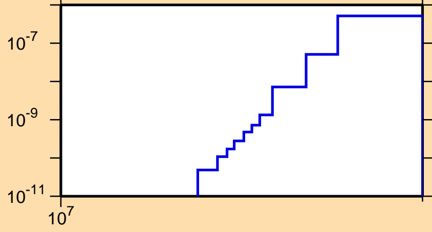
\sigma vs. E for ^{231}\text{Ra}(n,2n\alpha)
