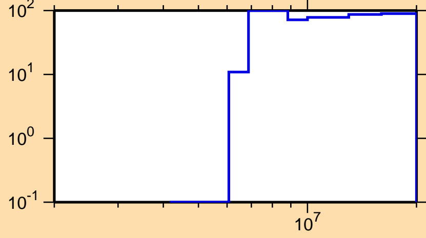
\Delta\sigma/\sigma vs. E for ^{231}\text{Ra}(n,p)
