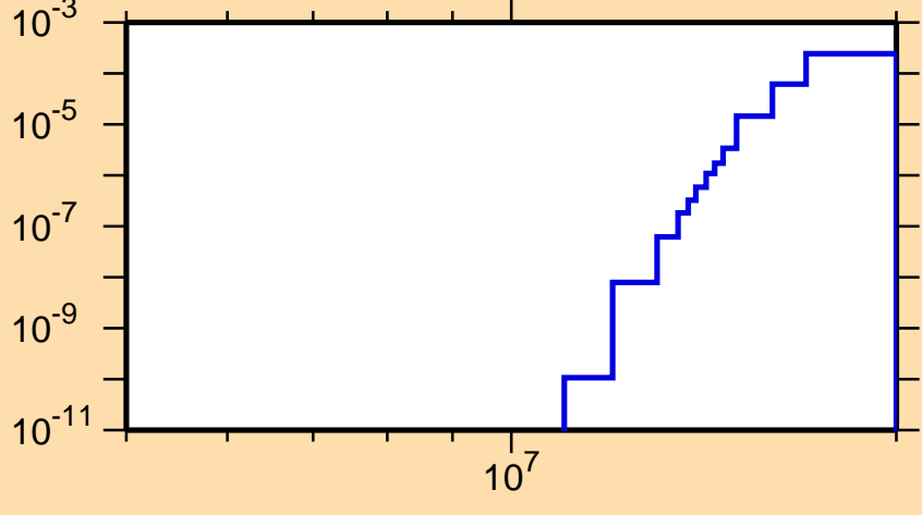
\sigma vs. E for ^{231}\text{Ra}(n,d)
