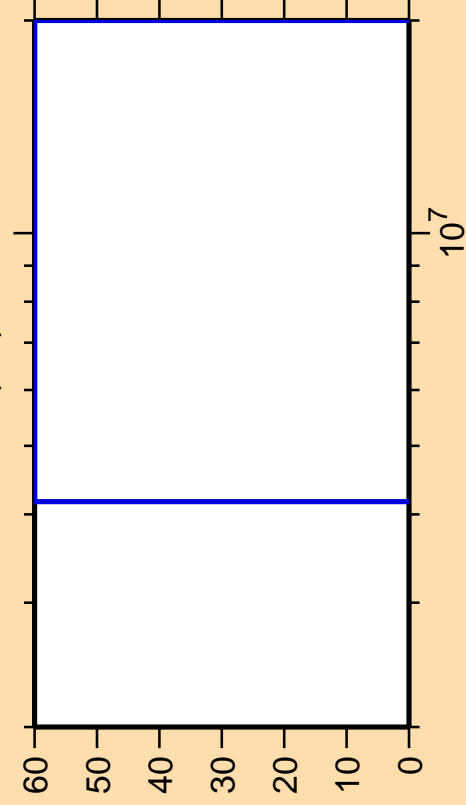
\Delta\sigma/\sigma vs. E for ^{231}\text{Ra}(n,f)
