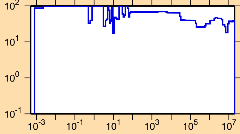
\Delta\sigma/\sigma vs. E for ^{231}\text{Ra}(n,\text{tot.})
