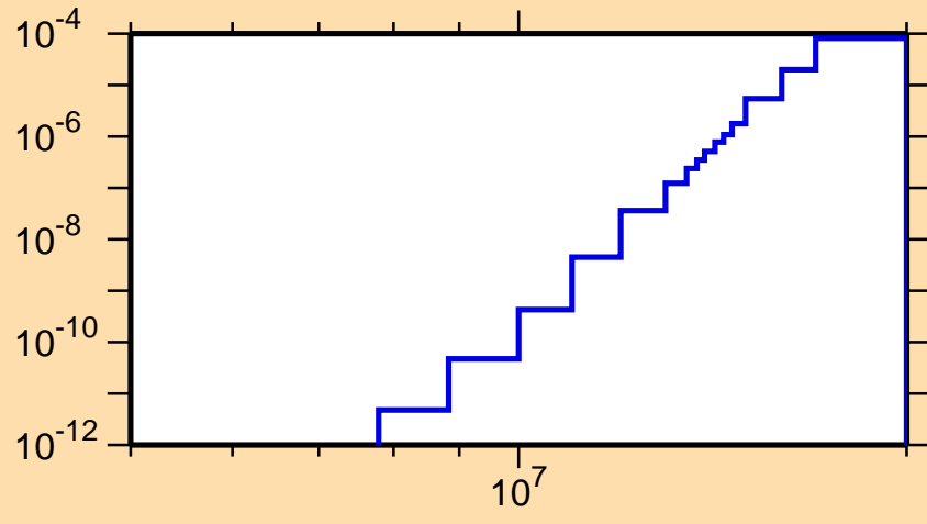
\sigma vs. E for ^{231}\text{Ra}(n,\alpha)
