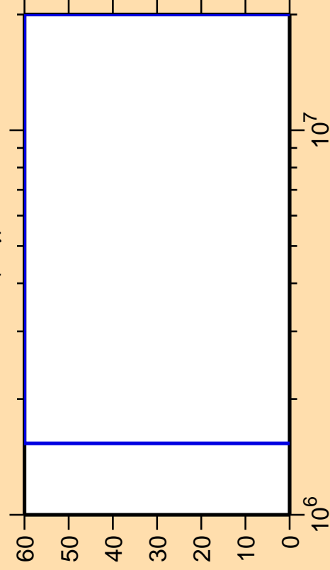
\Delta\sigma/\sigma vs. E for ^{231}\text{Ra}(n,\gamma)
