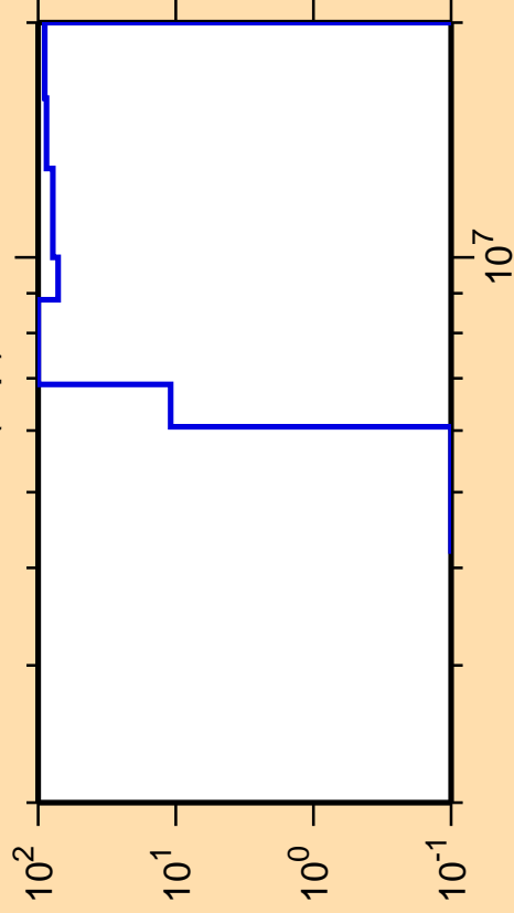
\Delta\sigma/\sigma vs. E for ^{231}\text{Ra}(n,p)
