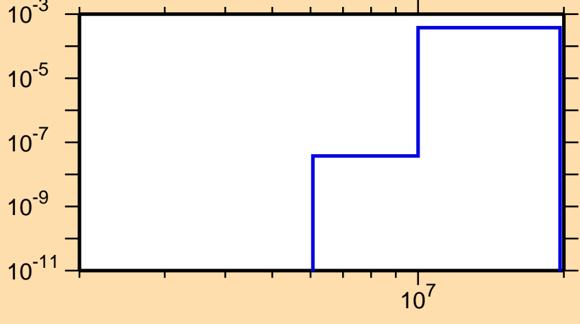
\sigma vs. E for ^{231}\text{Ra}(n,p)
