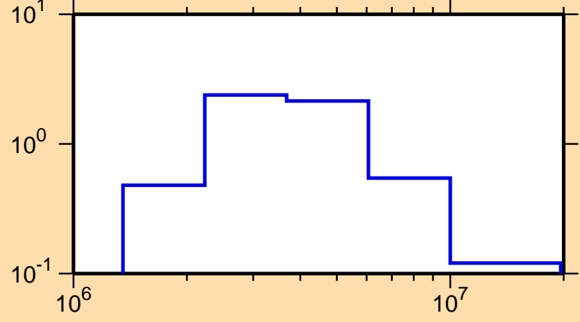
\sigma vs. E for ^{231}\text{Ra}(n,n\text{cont.})
