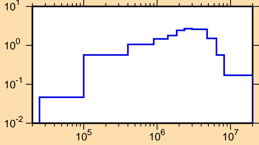
\sigma vs. E for ^{231}\text{Ra}(n,\text{inel.})
