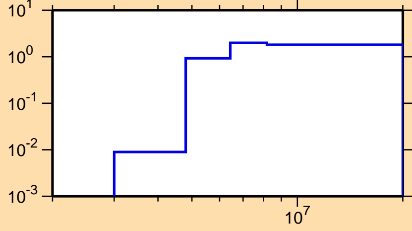
\sigma vs. E for ^{231}\text{Ra}(n,2n)
