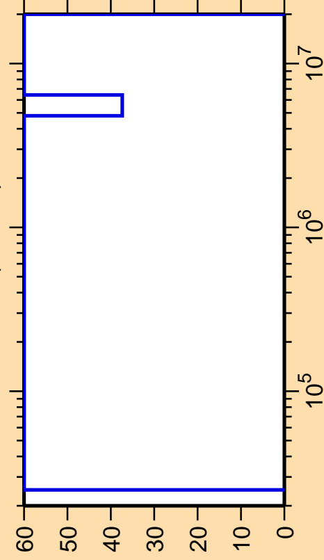
\Delta\sigma/\sigma vs. E for ^{231}\text{Ra}(n,\text{inel.})
