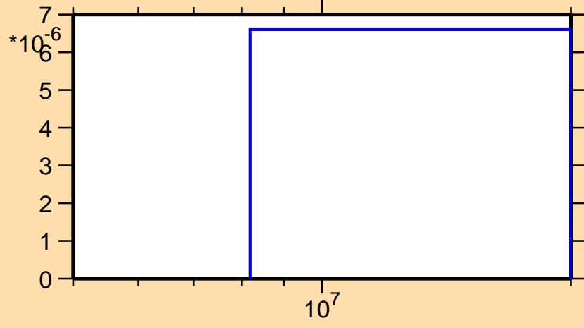
\sigma vs. E for ^{231}\text{Ra}(n,d)
