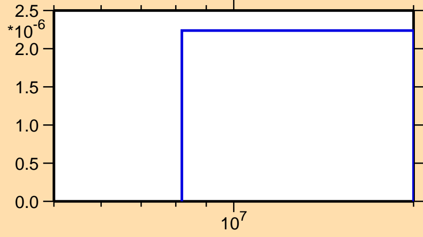
\sigma vs. E for ^{231}\text{Ra}(n,np)
