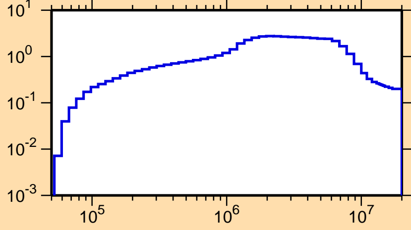
\sigma vs. E for ^{232}\text{Ra}(n,\text{inel.})
