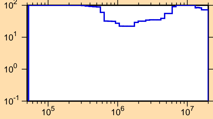
\Delta\sigma/\sigma vs. E for ^{232}\text{Ra}(n,\text{inel.})
