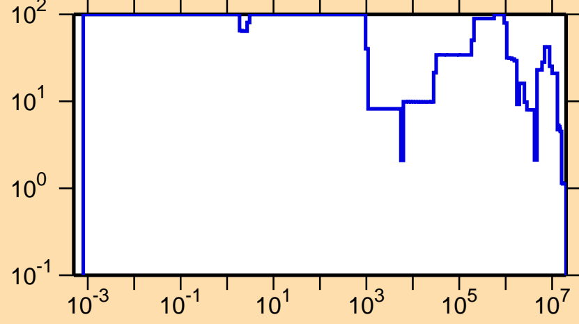
\Delta\sigma/\sigma vs. E for ^{232}\text{Ra}(n,\text{el.})
