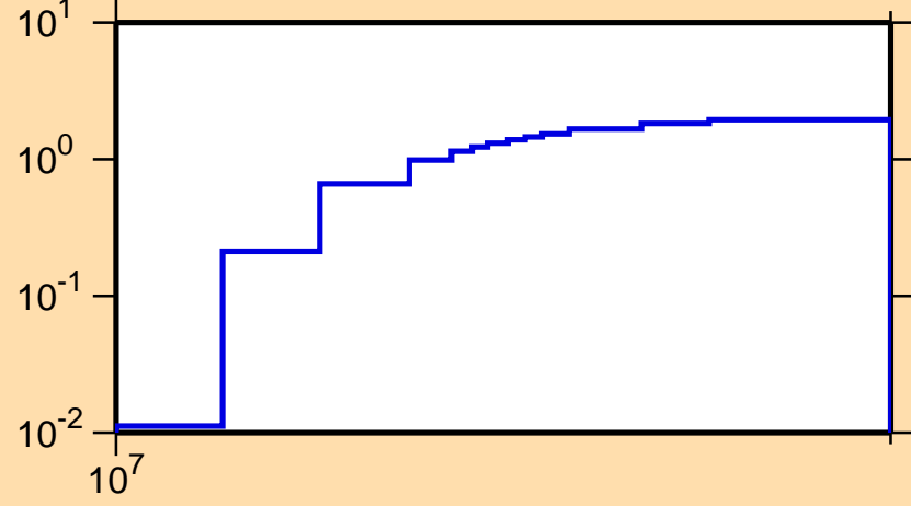
\sigma vs. E for ^{232}\text{Ra}(n,3n)
