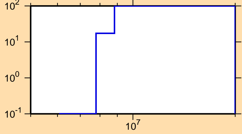
\Delta\sigma/\sigma vs. E for ^{232}\text{Ra}(n,p)
