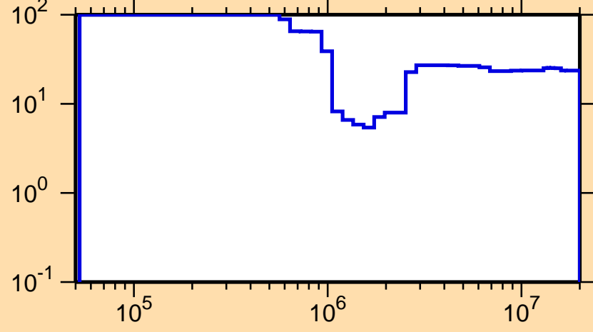
\Delta\sigma/\sigma vs. E for ^{232}\text{Ra}(n,\text{nonel.})
