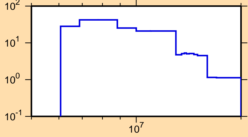
\Delta\sigma/\sigma vs. E for ^{232}\text{Ra}(n,el.)
