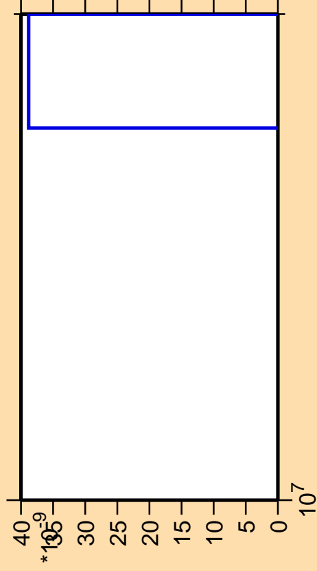
\Delta\sigma/\sigma vs. E for ^{232}\text{Ra}(\text{mt } 42)
