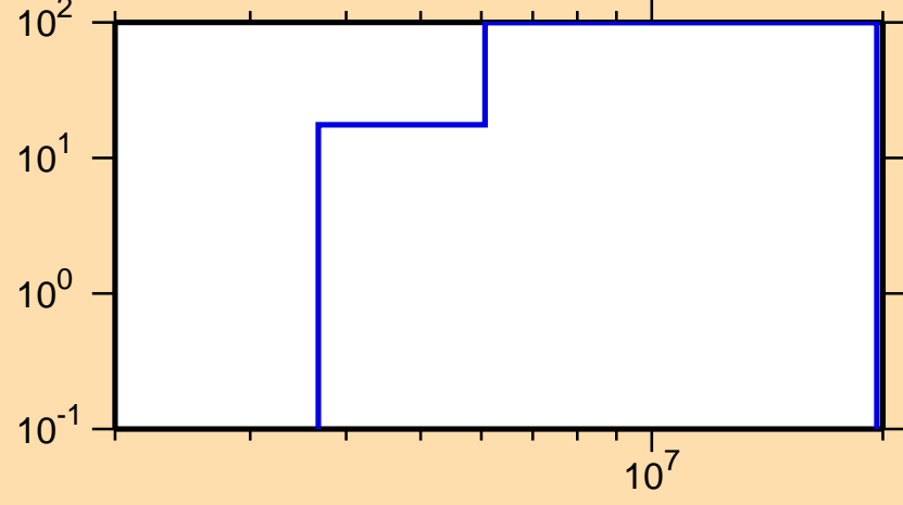
\Delta\sigma/\sigma vs. E for ^{232}\text{Ra}(n,\gamma)
