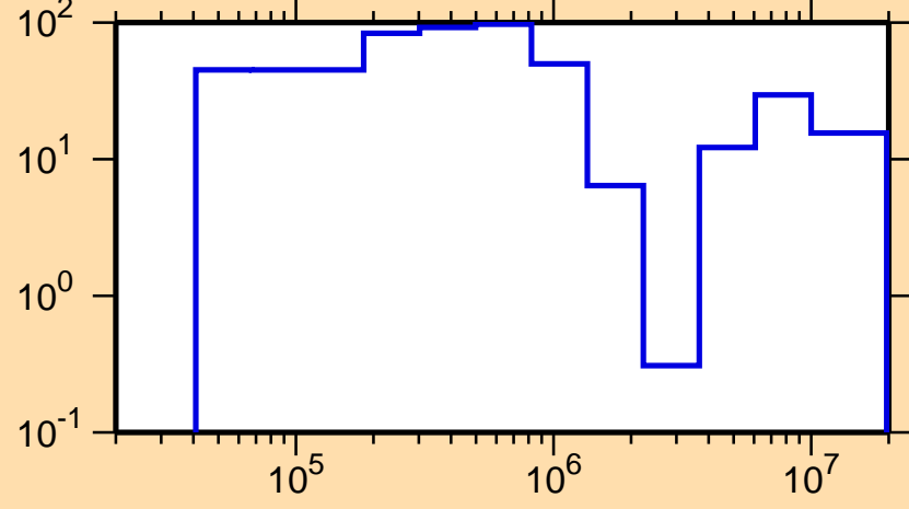
\Delta\sigma/\sigma vs. E for ^{232}\text{Ra}(n,\text{tot.})
