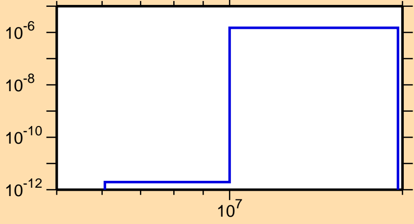
\sigma vs. E for ^{232}\text{Ra}(n,n\alpha)
