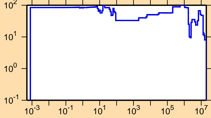
\Delta\sigma/\sigma vs. E for ^{233}\text{Ra}(n,\text{el.})
