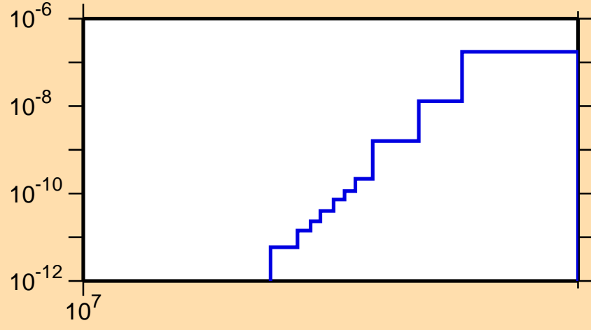
\sigma vs. E for ^{233}\text{Ra}(n,2n\alpha)
