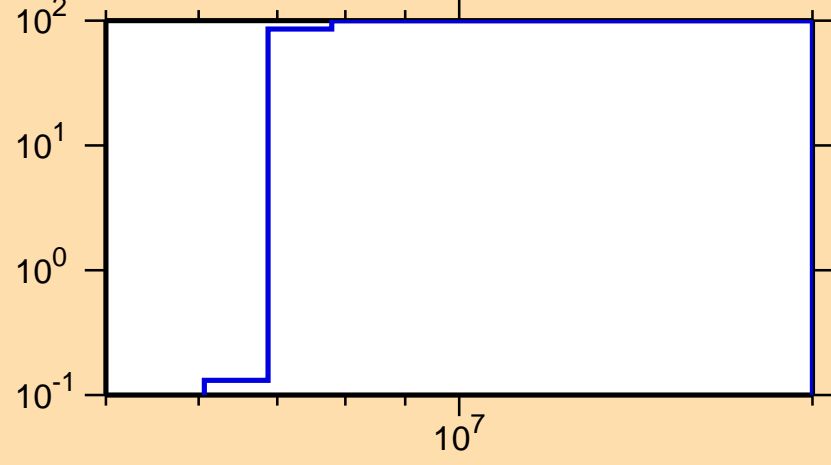
\Delta\sigma/\sigma vs. E for ^{233}\text{Ra}(n,p)
