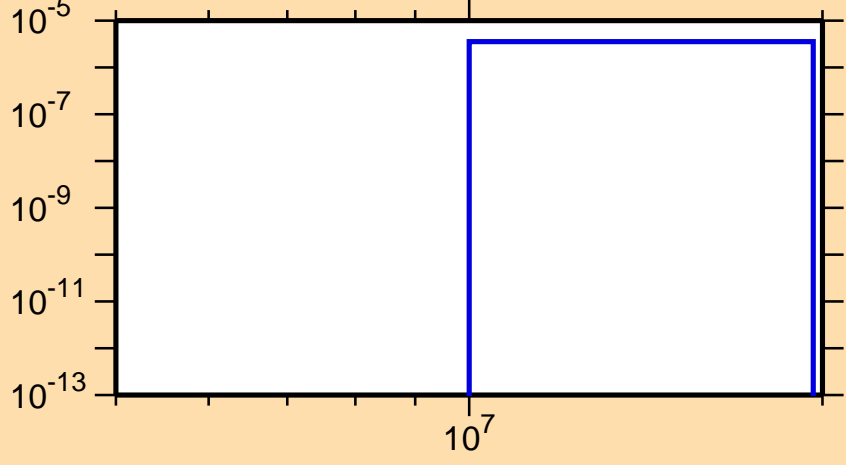
\sigma vs. E for ^{233}\text{Ra}(n,d)
