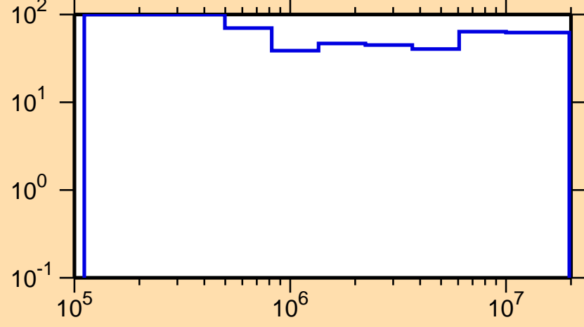
\Delta\sigma/\sigma vs. E for ^{233}\text{Ra}(n,\text{inel.})
