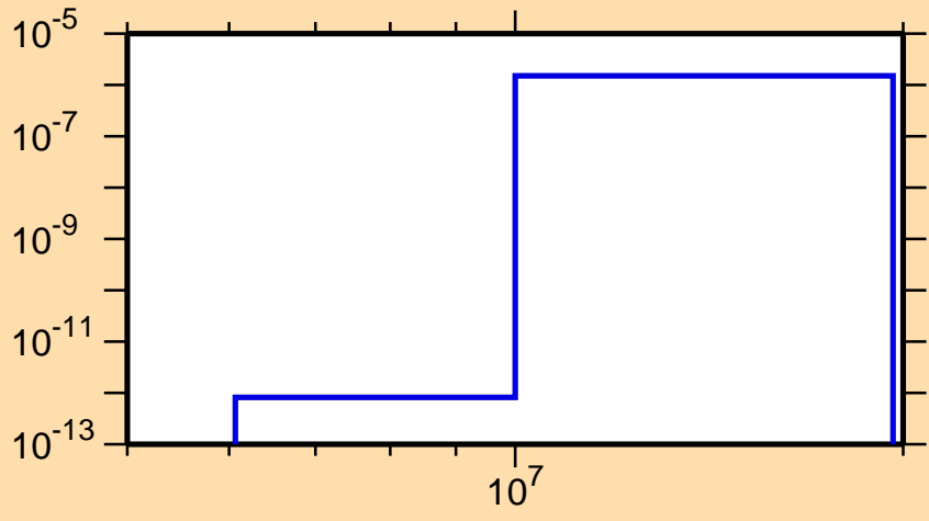
\sigma vs. E for ^{233}\text{Ra}(n,\alpha)
