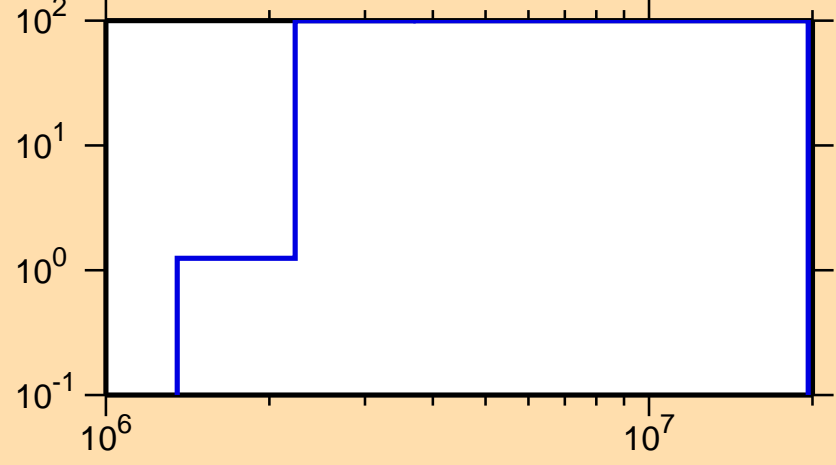
\Delta\sigma/\sigma vs. E for ^{233}\text{Ra}(n,f)
