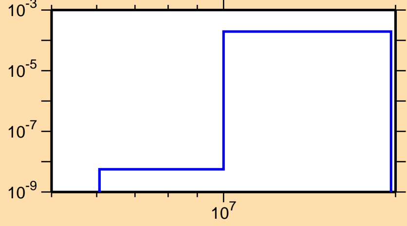
\sigma vs. E for ^{233}\text{Ra}(n,p)
