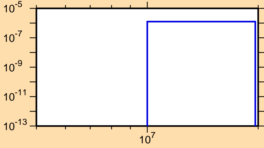
\sigma vs. E for ^{233}\text{Ra}(n,np)
