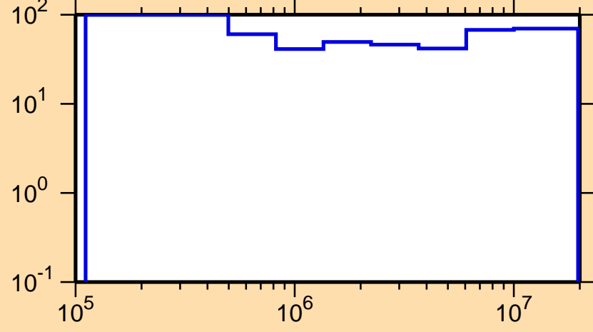
\Delta\sigma/\sigma vs. E for ^{233}\text{Ra}(n,ncont.)
